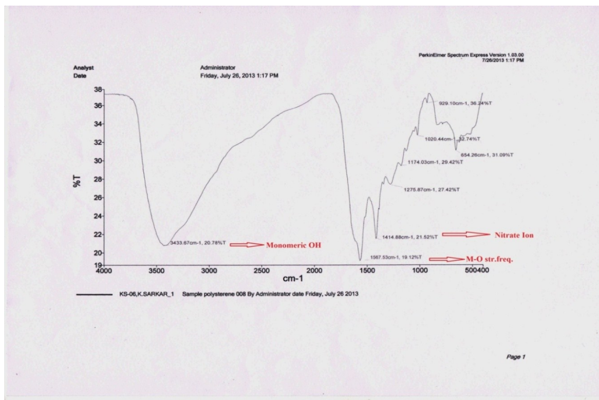
Figure S2: Infra red spectrum of Ag-Morin complex
