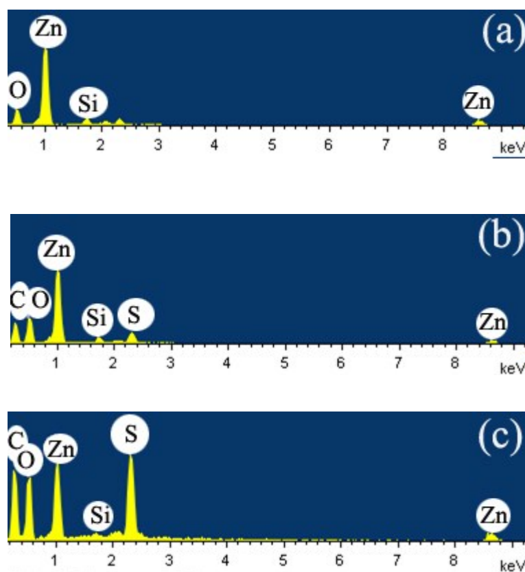
Figure.S1 EDS patterns of the typical productions with SDS concentrations of (a) 0.5mM, (b) 25mM, (c) 50 mM, respectively.
