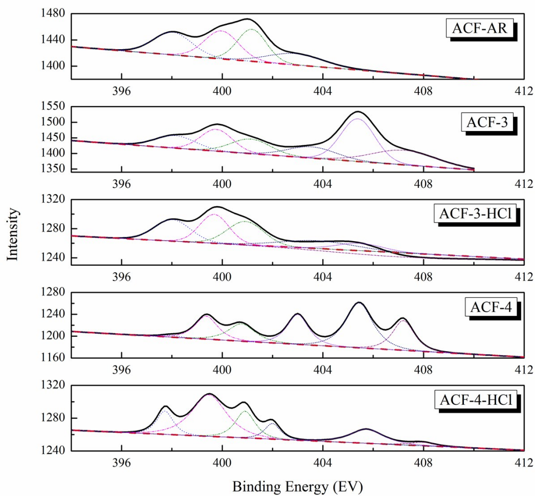
N_{1s} subpeaks of XPS spectra of the ACFs
