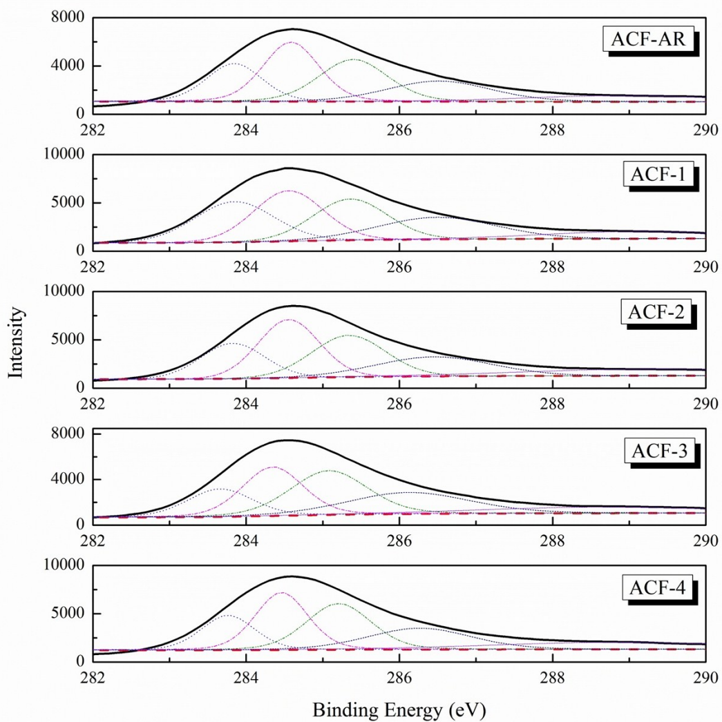
C 1s subpeaks of XPS spectra of the ACFs
