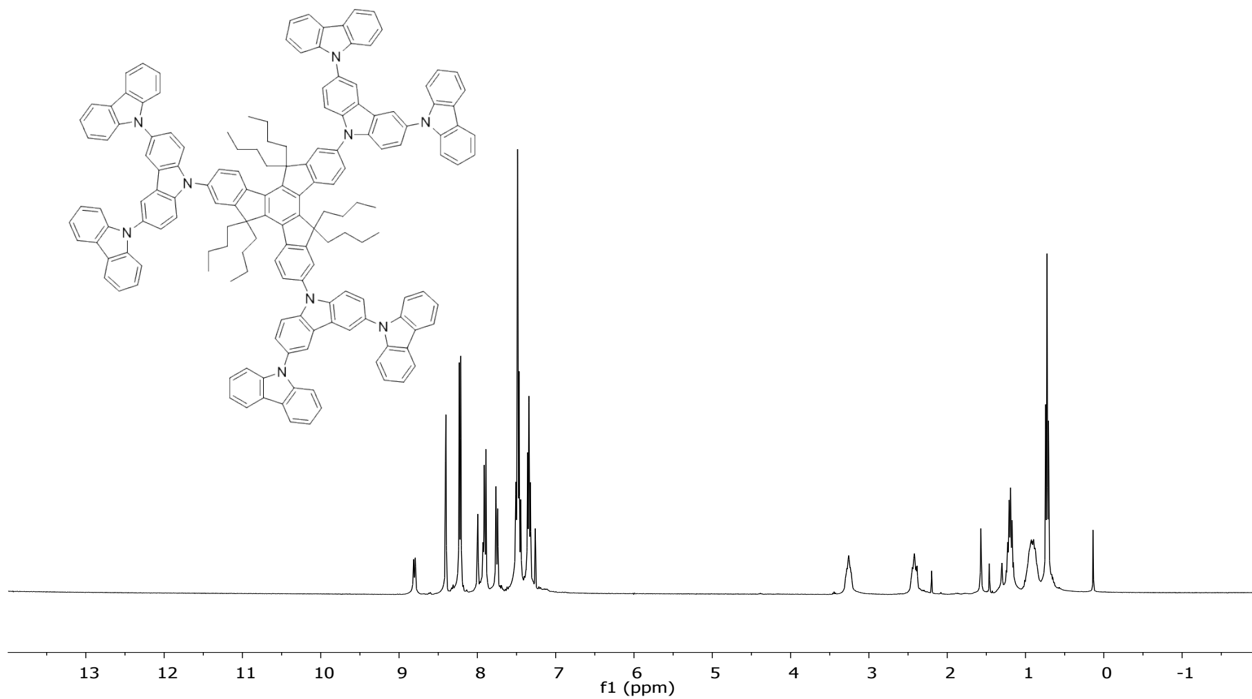
Figure S3 ^1\text{H-NMR} spectrum of 2 in \text{CDCl}_3
