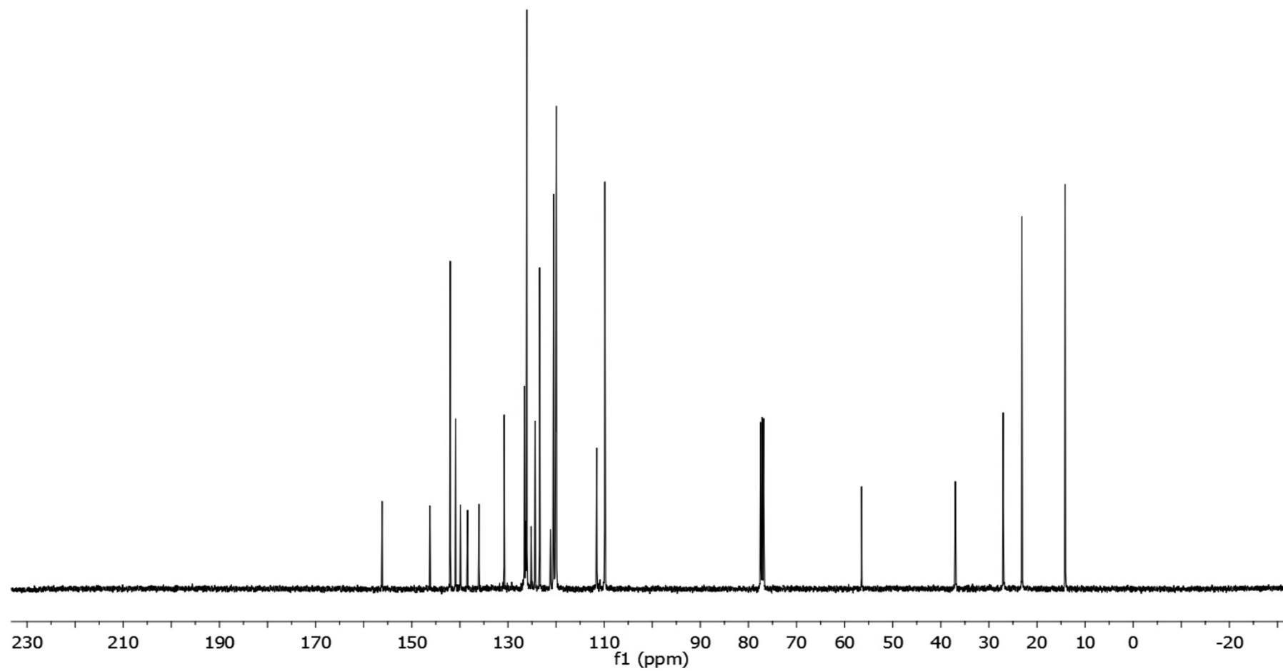
Figure S4 ^{13}\text{C} -NMR spectrum of 2 in \text{CDCl}_3
