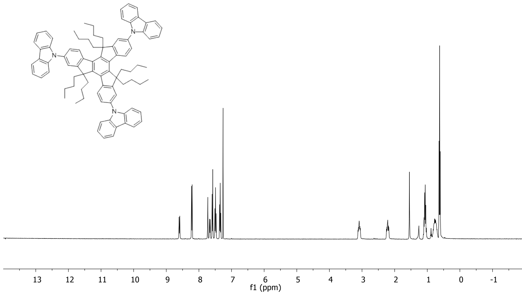
Figure S1 1 H-NMR spectrum of 1 in CDCl 3
