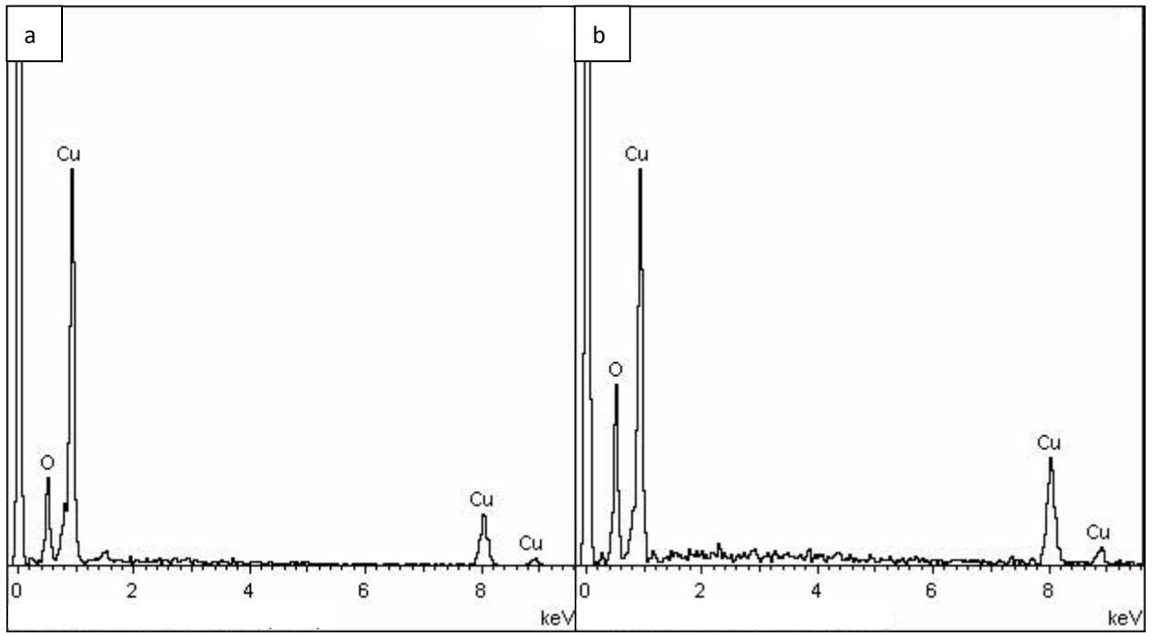
Figure S2. EDS spectrums of site 1 (a) and site 2 (b) in Fig. 3c.
