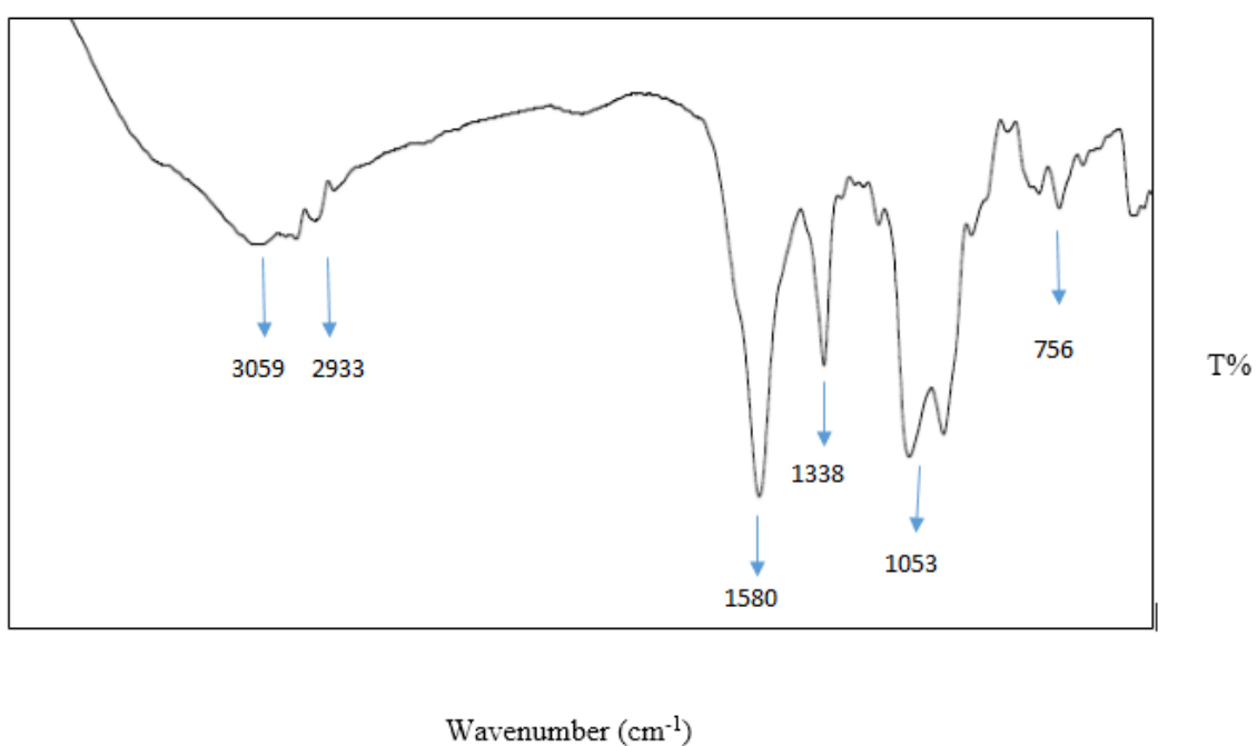
Fig. S1. FT-IR spectrum of SiC-dots.
