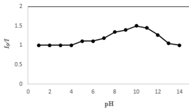
Fig. S3. Effects of pH the on the fluorescence changes of sensor
