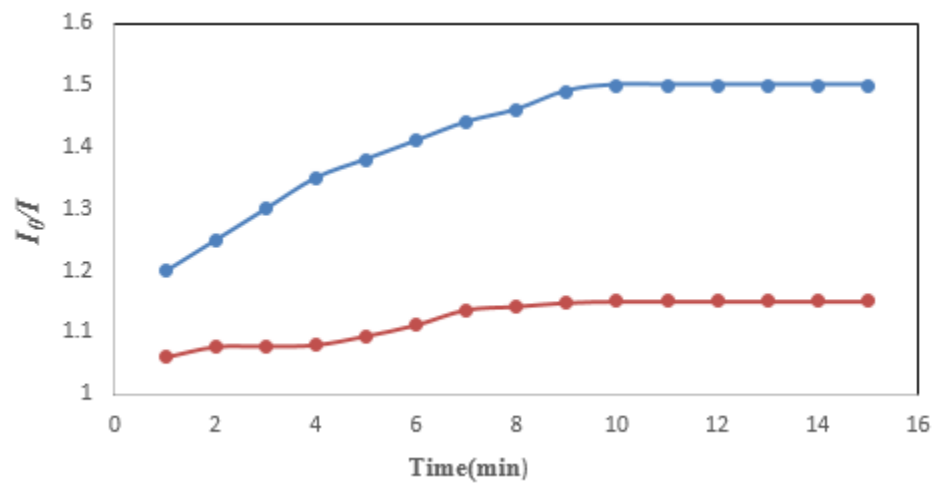
Fig. S4. Kinetic uptake of NIF molecules on to MIP@SiC-dots (blue), NIP@SiC-dots (red).
