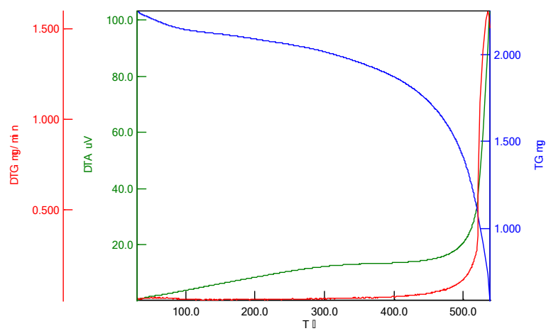
Fig. S1 TGA curve of graphene stationary phase using Shimadzu TGA-50H Thermoanalyzer.
