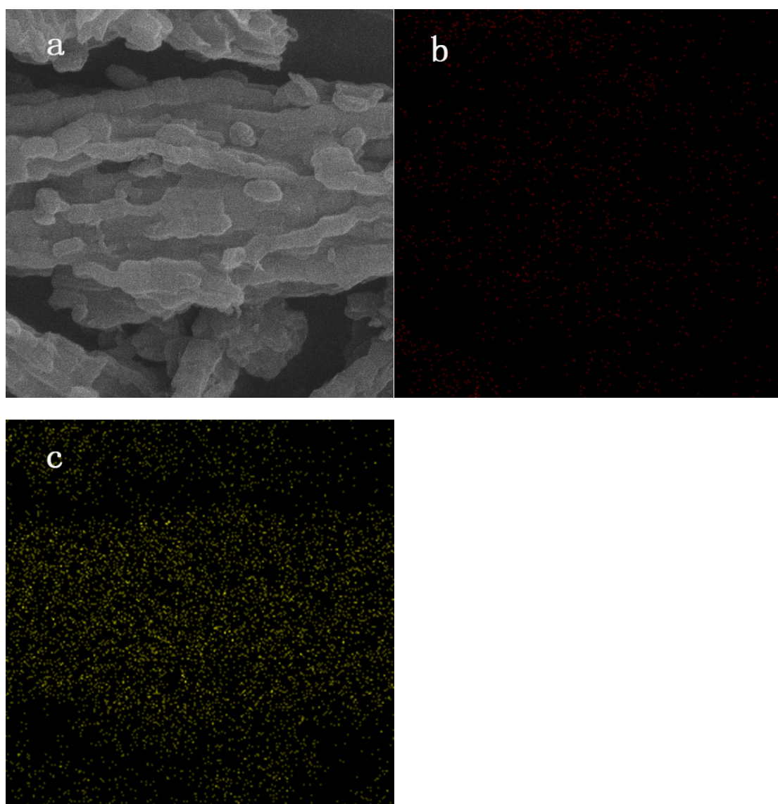
Fig. S1 (a) SEM images of CMK-3/S hybrids, elemental C (b) and S (c) maps of CMK-3/S composite from (a).
