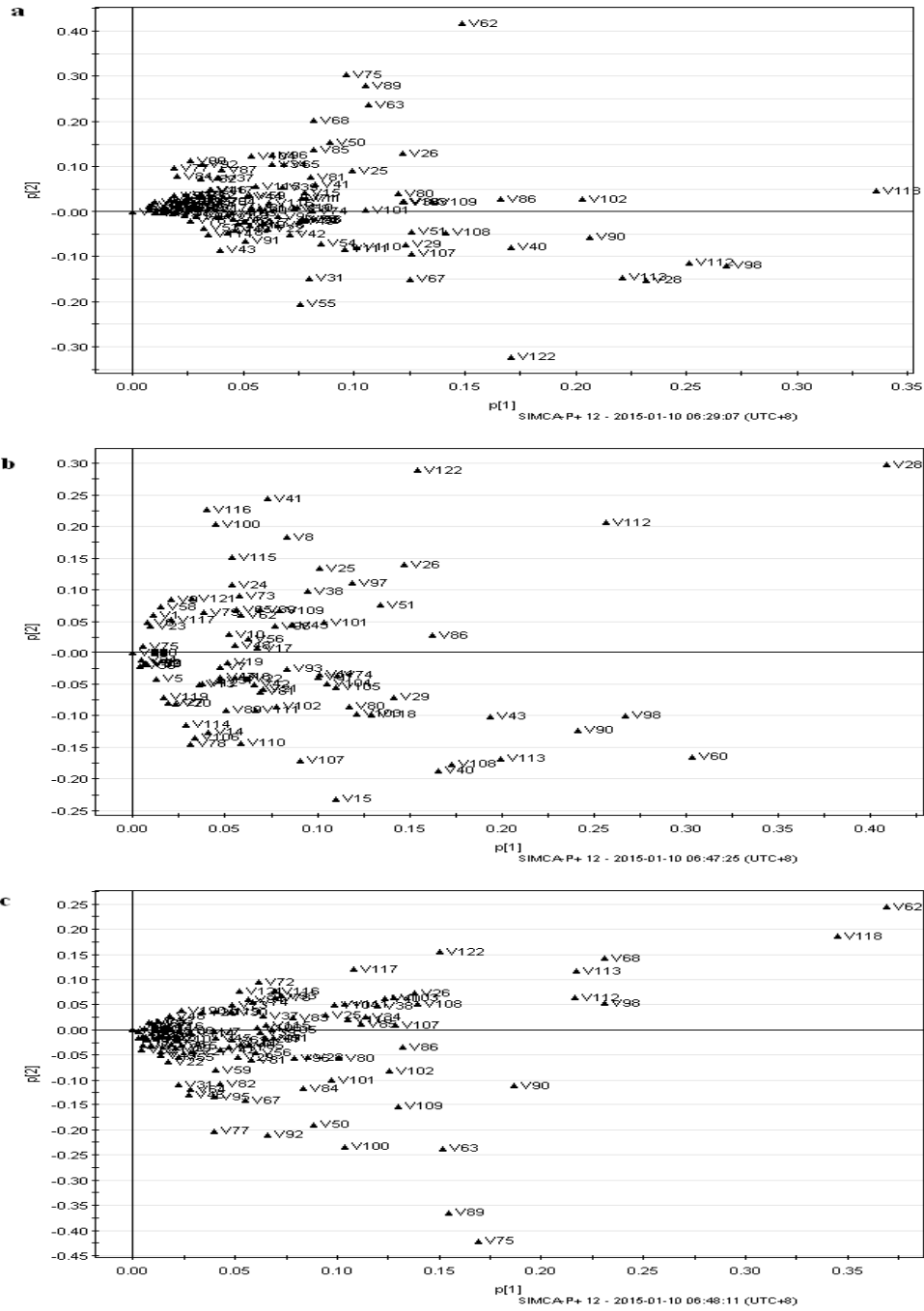
Figure S2 The loading plots of different years aged tea (a), raw tea (b) and ripe tea (c)
