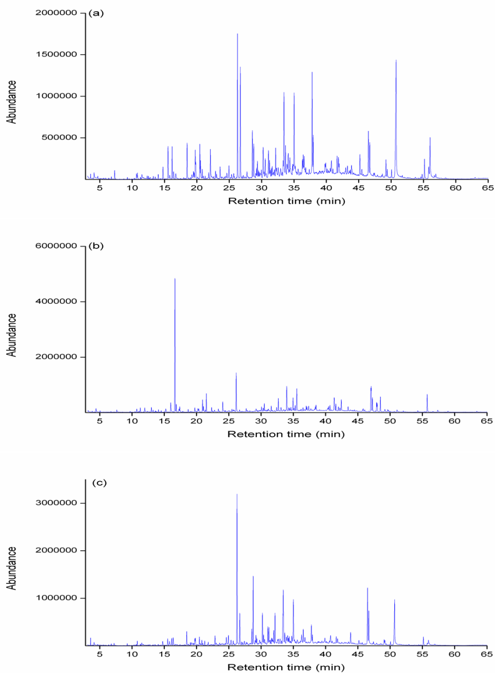
Figure S1 Total ion chromatograms of Pu-erh tea by HS-SPME/GC-MS (a aged tea, b raw tea, c ripe tea)
