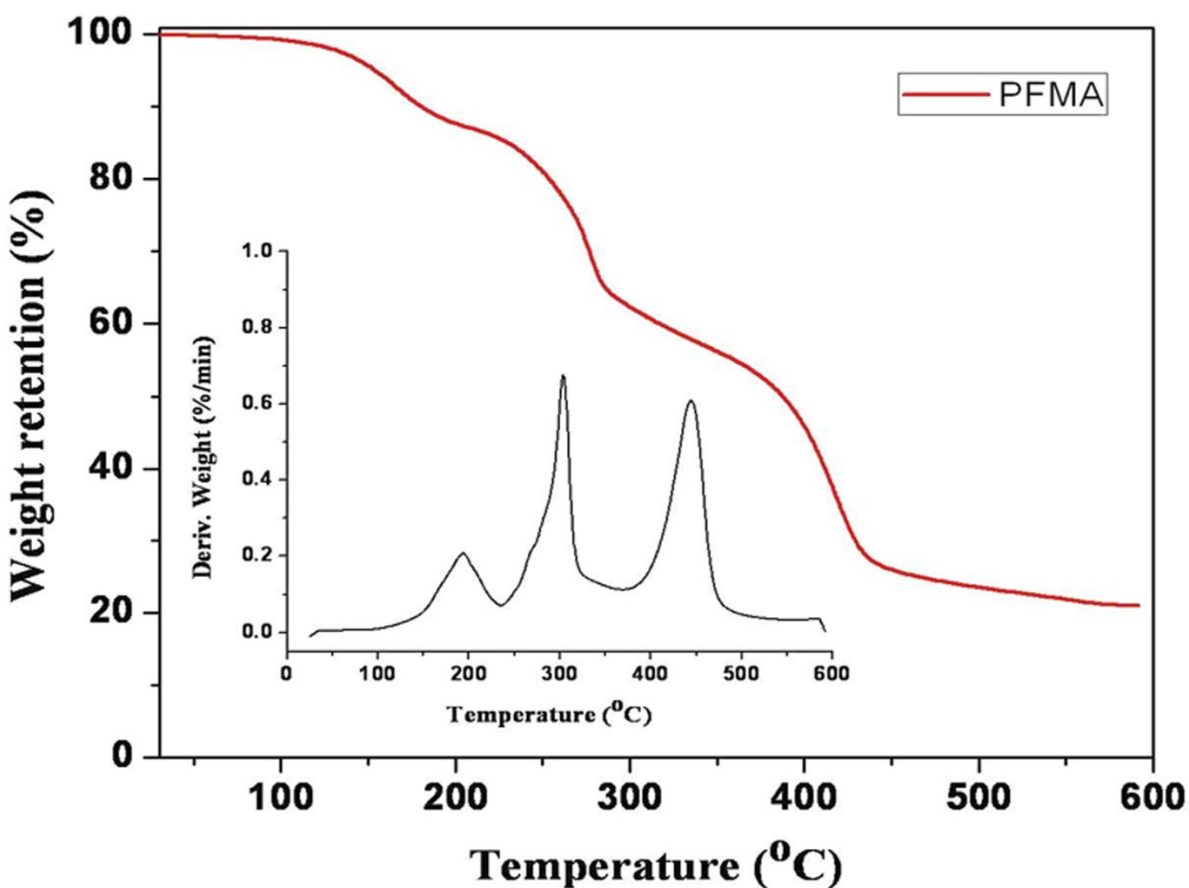
Figure S1. TGA and DTG thermogram of PFMA prepared via RAFT polymerization.
