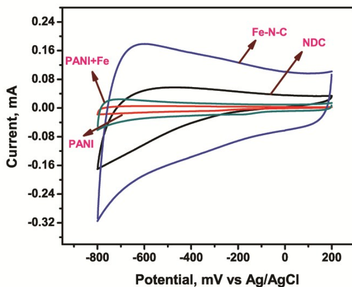
Figure S1: CV curves of respective electrocatalyst in 0.1 M KOH electrolyte, at scan rate 10 \text{mV/s}^{-1}
