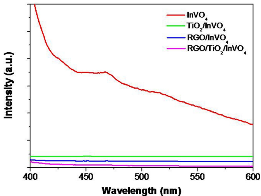
Fig. S2 Room temperature PL spectra of as-synthesized samples under the excitation wavelength of 325 nm.
