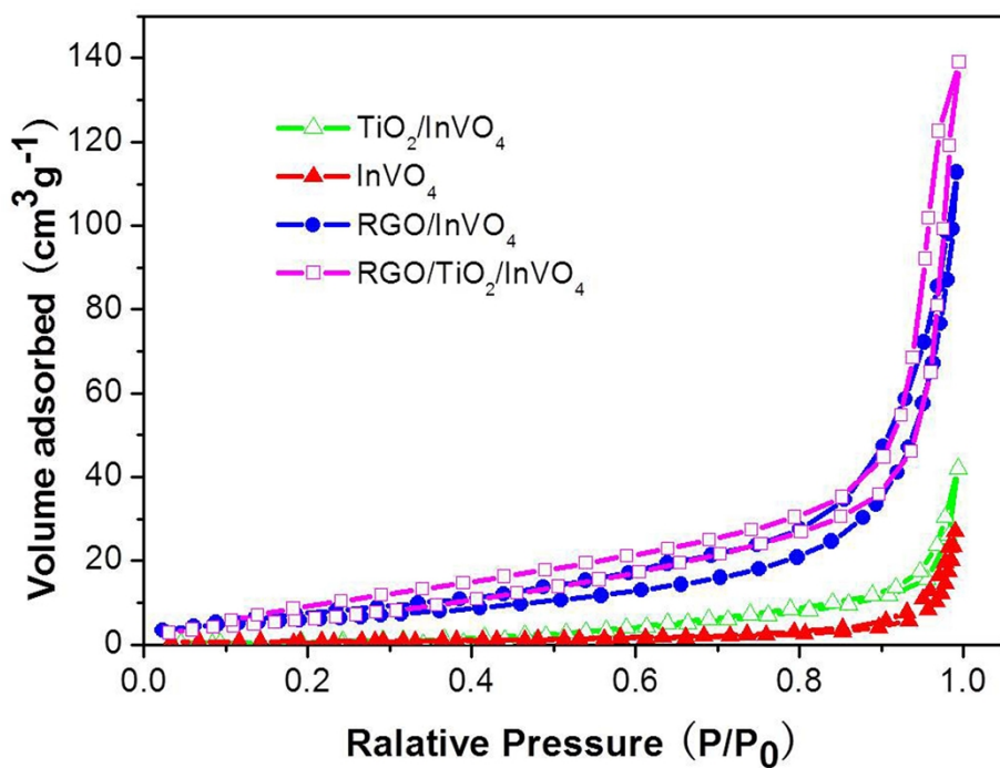
Fig. S1 N 2 adsorption-desorption isotherm curves of the as-prepared samples.
