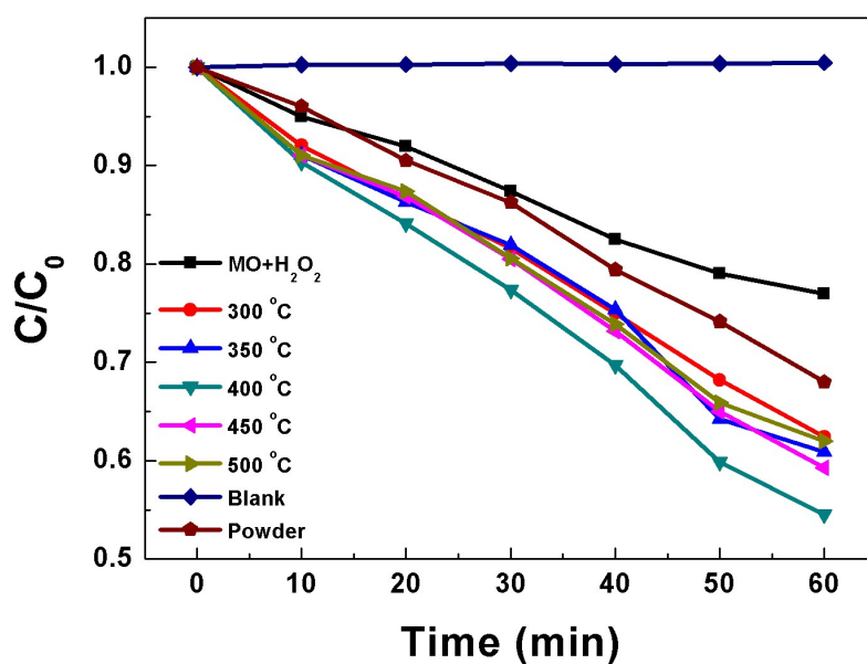
Figure S1. Degradation curve of methyl orange of \alpha -Fe 2 O 3 nanopillars and powder samples
