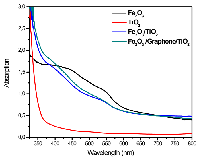
Figure S1 UV-Vis absorption spectra of \alpha\text{-Fe}_2\text{O}_3 , \text{TiO}_2 , \alpha\text{-Fe}_2\text{O}_3/\text{TiO}_2 and \alpha\text{-Fe}_2\text{O}_3/\text{Graphene}/\text{TiO}_2 photoanodes
