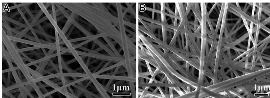
Fig. S1. SEM images of (A) electrospun PAN nanofibers, (B) glutaral-functional PAN nanofibers.
