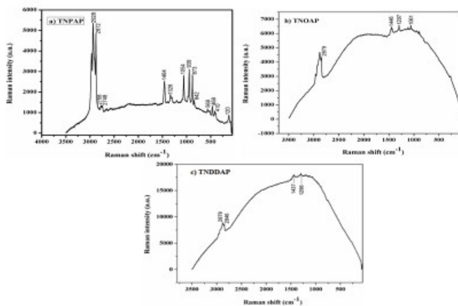
Fig. 2: Dispersive Raman spectra of a) TNPAP, b) TNOAP and c) TNDDAP.
