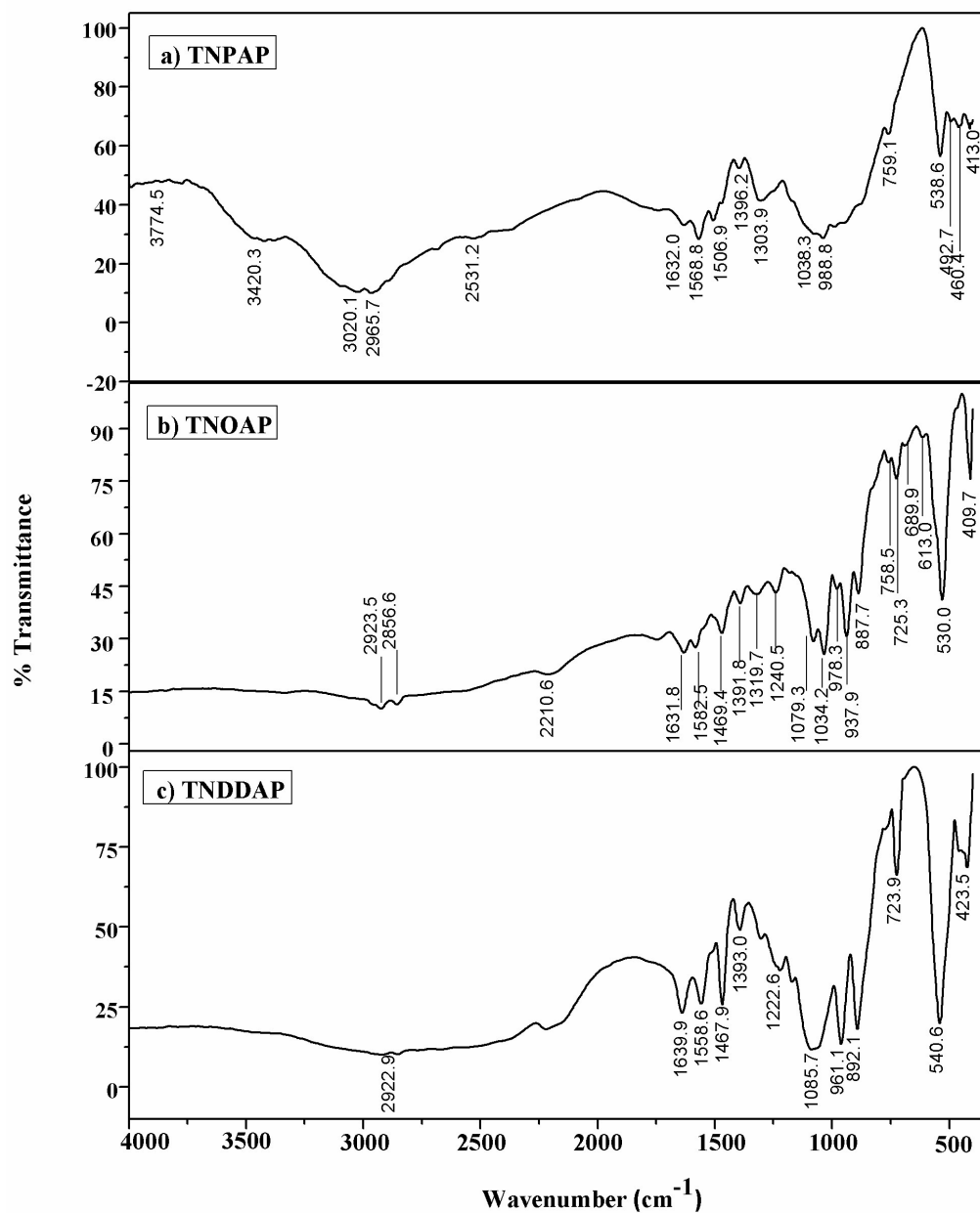
Fig. 1: Fourier transform Infra red of a) TNPAP, b) TNOAP and c) TNDDAP.
