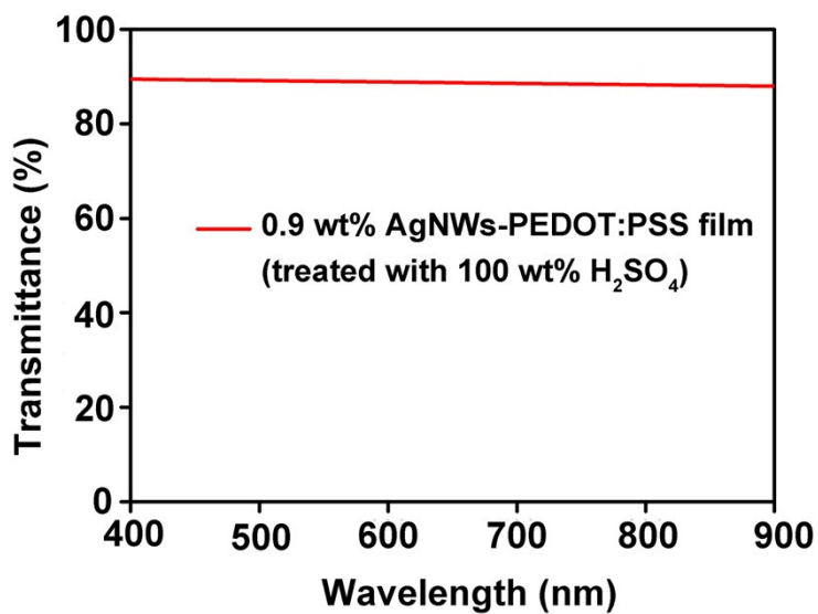
Fig. S2. Optical transmittance spectra of 0.9 wt% AgNWs-PEDOT:PSS composite film treated with 100 wt% H 2 SO 4 .
