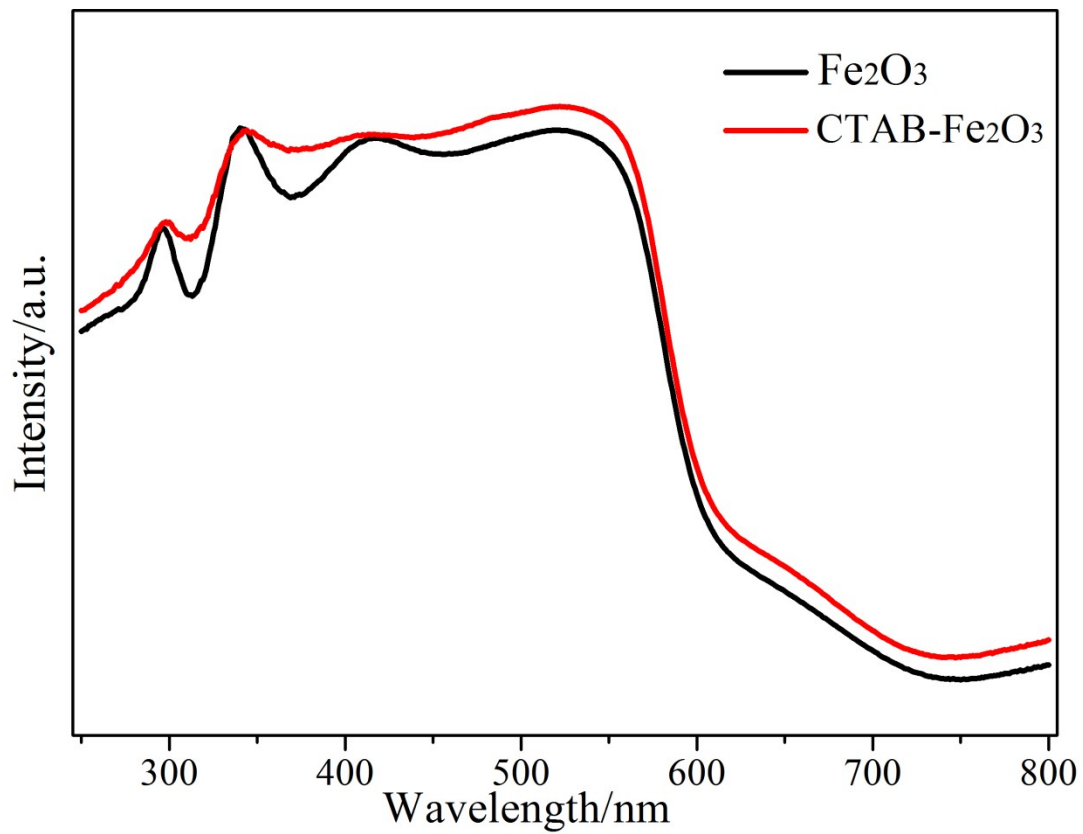
Fig. S3 UV-vis absorption spectra of Fe 2 O 3 and CTAB-Fe 2 O 3 .
