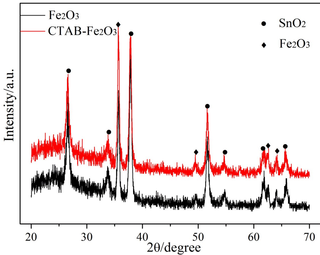
Fig. S1 XRD patterns of Fe 2 O 3 and CTAB-Fe 2 O 3 .
