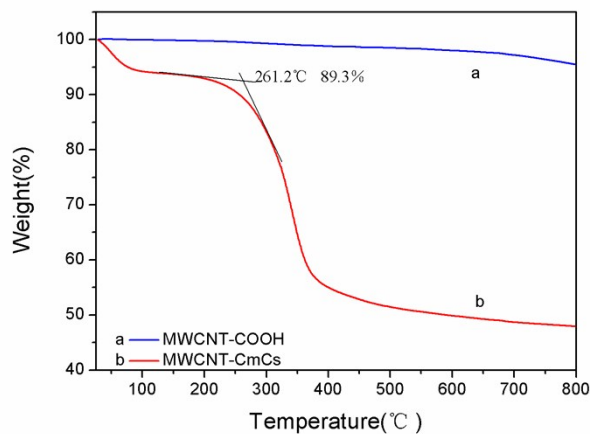
Fig.S2 TGA traces of MWCNT-COOH (a), and MWCNT-CmCs (b)
