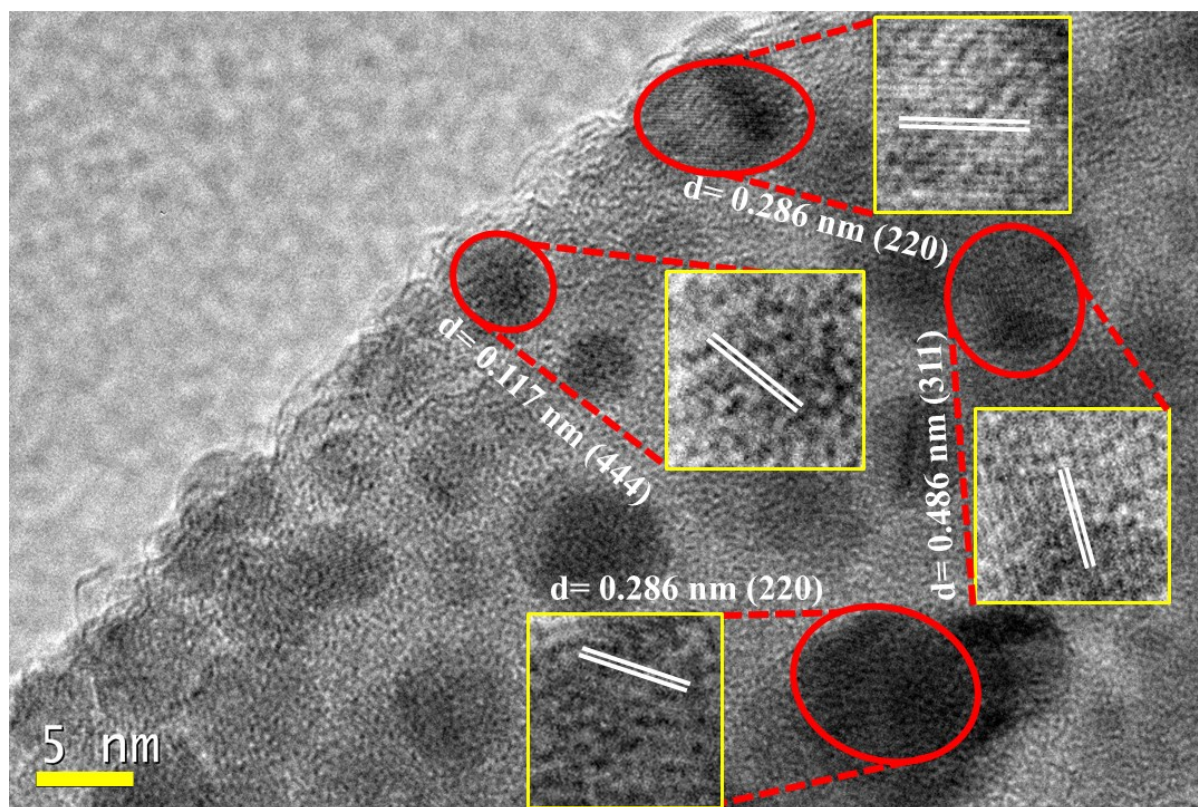
Fig. 2 High resolution TEM images of ZCO/rGO hybrid composites..
