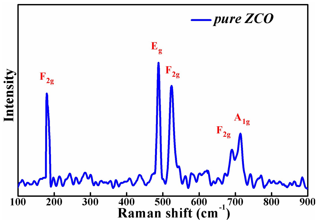
Fig. 1 Raman spectrum of pure ZCO materials.
