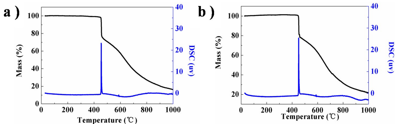
Fig. S2 TG-DSC curves of the (a) large-sized and (b) small-sized crystals of ZIF-71
