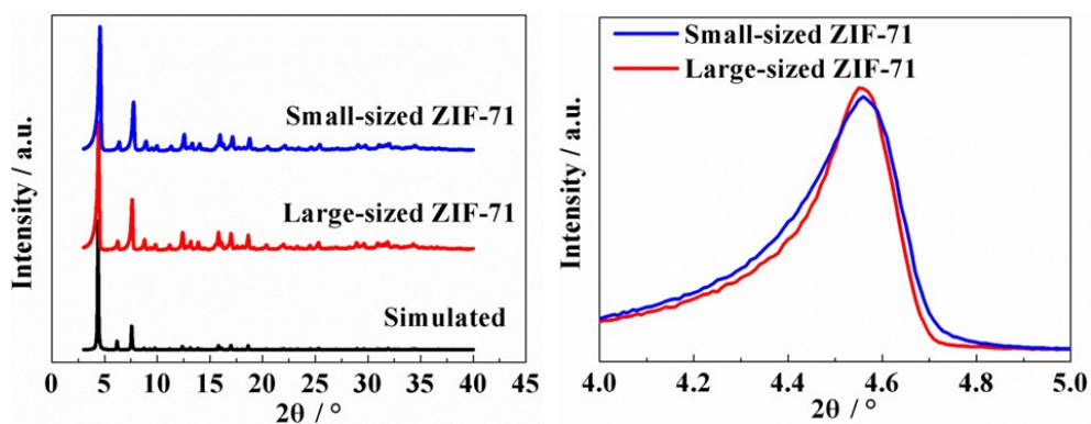
Fig. S3 PXRD pattern of the ZIF-71 product compared with the simulated ZIF-71 pattern (The right is partial enlarged detail).
