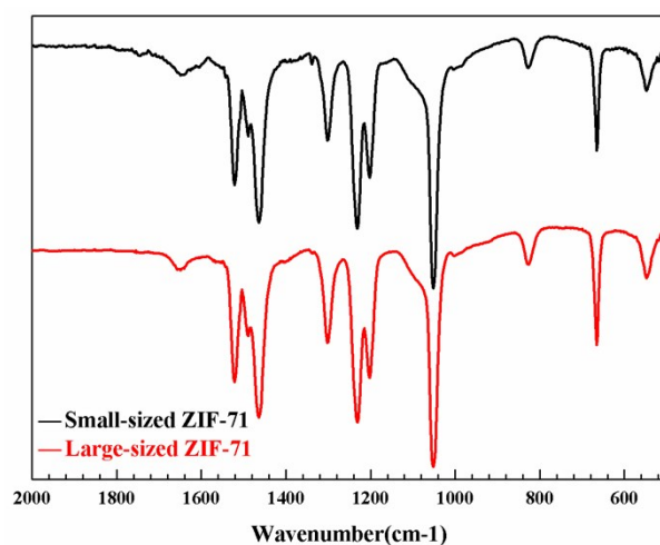
Fig. S1 FT-IR of small- and large-sized crystals of ZIF-71
