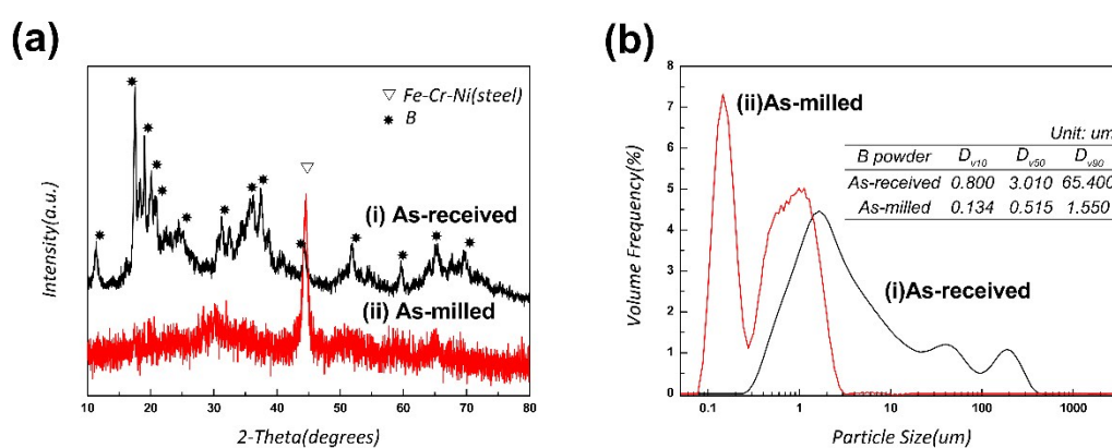
Fig. S2 (a) The XRD patterns and (b) particle size distribution of as-received and as-milled boron powder. The table inserted in the right figure presents D v10 , D v50 and D v90 values of as-received and as-milled boron powder.
