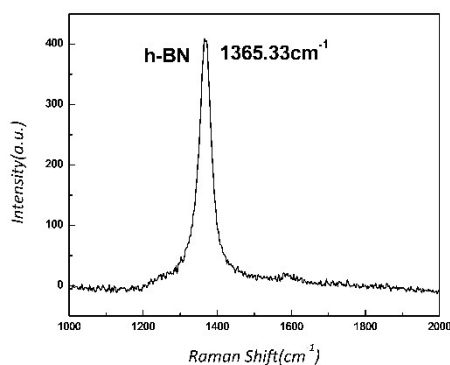
Fig. S1 Raman spectra of the as-grown BNNTs.
