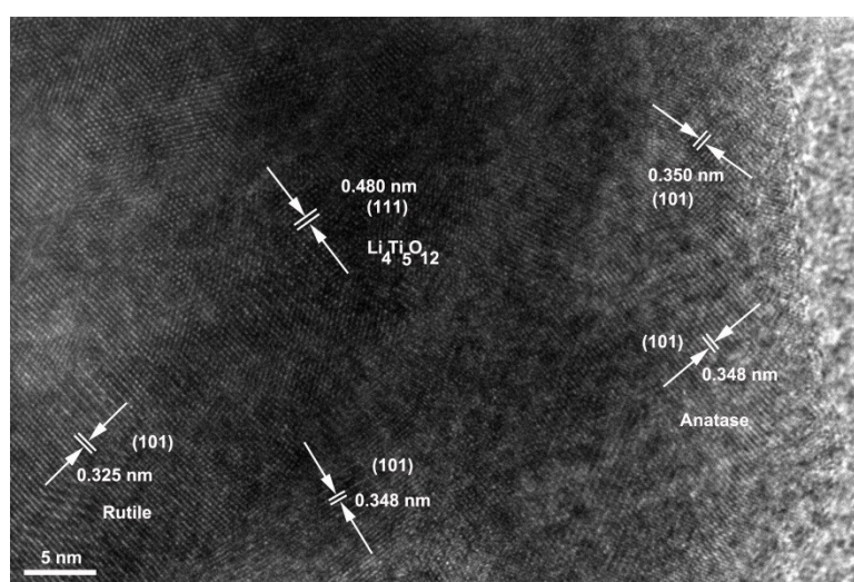
Fig. S1 Typical high-resolution TEM image of \text{Li}_4\text{Ti}_5\text{O}_{12} - \text{TiO}_2 composite.
