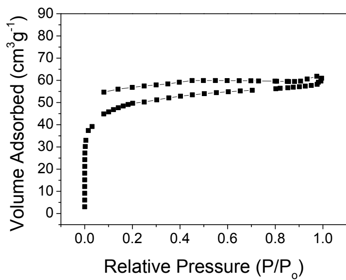
Fig. S1 Nitrogen adsorption-desorption isotherms of GO (100 mesh) by rapid freeze-drying.
