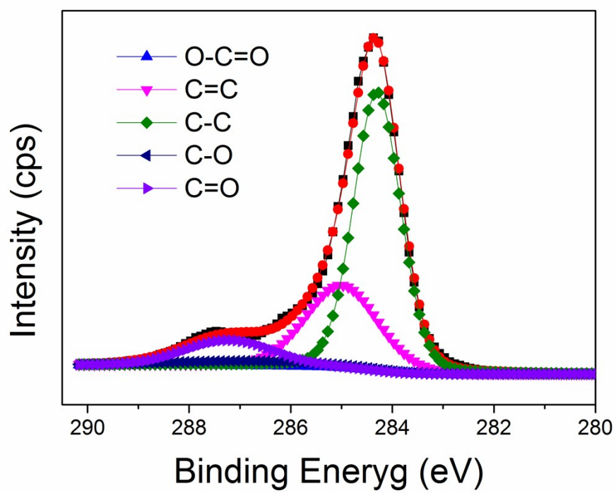
Fig. S2 XPS spectra of C1s in GO (100 mesh) after 1500 cycles.
