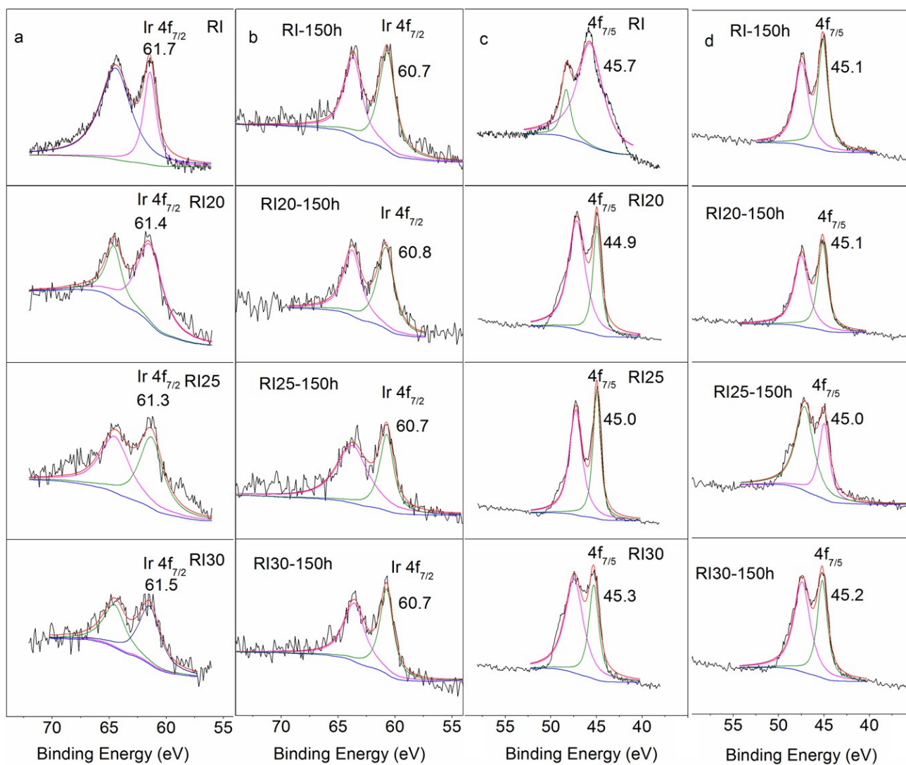
Figure S1 Ir and Re 4f XPS spectra for the RI, RI20, RI25 and RI30 samples. (a) Ir before reaction. (b) Ir after reaction. (c) Re before reaction. (d) Re after reaction.
