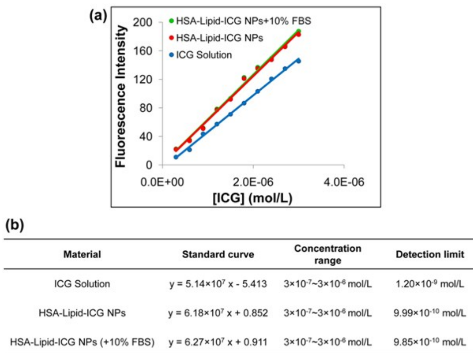
FIG. S2. (a) The standard curves and (b) the details of the calculation of ICG solution, HSA-Lipid-ICG NPs in PBS and HSA-Lipid-ICG NPs in PBS containing 10% FBS..
