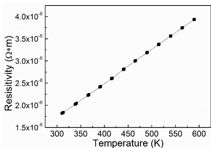
Figure S1. Temperature dependence electrical resistivity for WP_2
