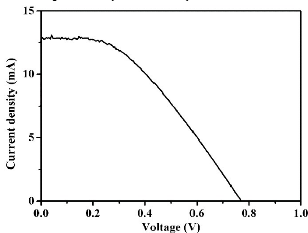
Fig. S2. Photocurrent–voltage curves of the DSSCs with rGO.
