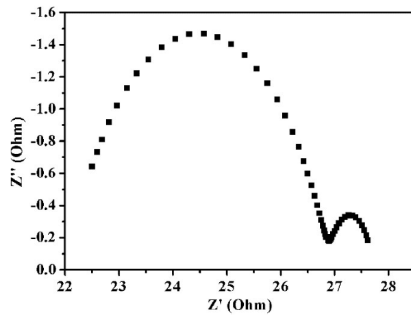
Fig.S4. Nyquist plots of the symmetrical cells fabricated with rGO.
