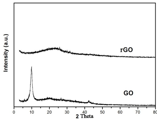
Fig. S1. XRD patterns of sample: rGO and GO.
