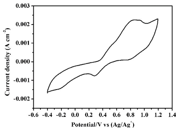
Fig.S3. Cyclic voltammograms of the triiodide/iodide redox couple for rGO.
