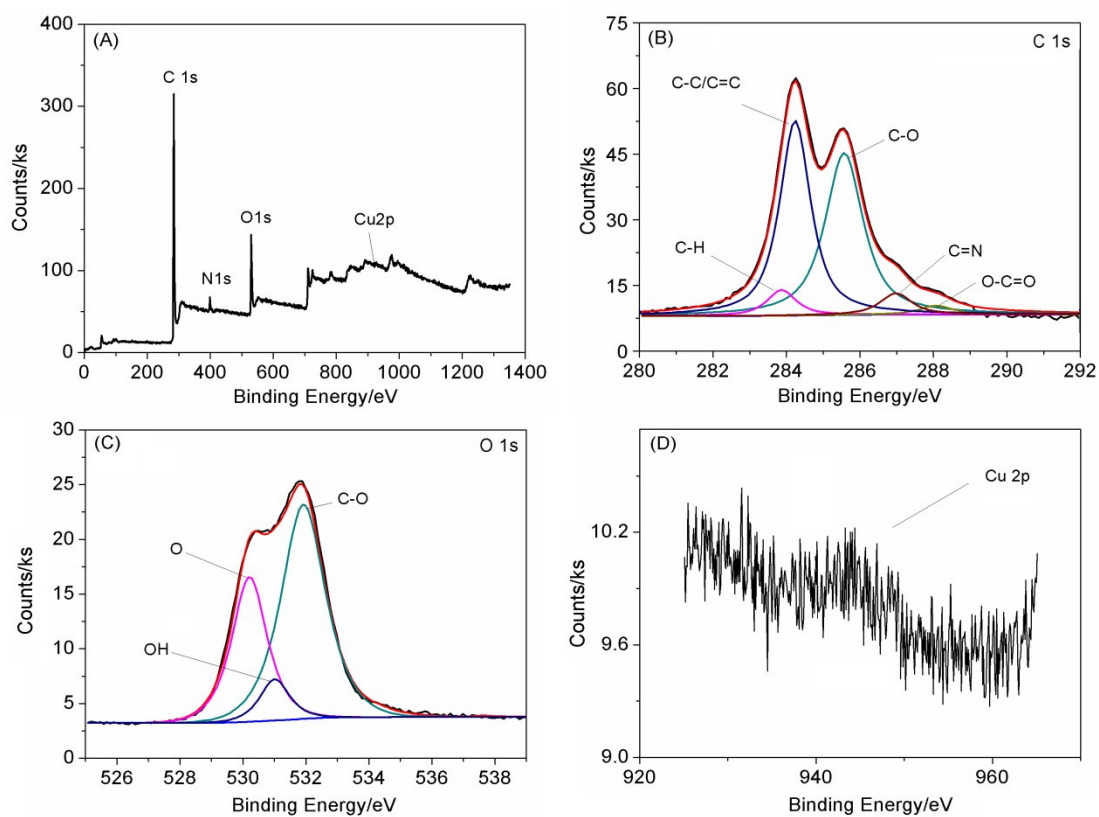
Fig. S1. XPS spectra of the Tyr-1-FP/rGO electrode: wide scan (A) and high resolution scans for C 1s (B), O 1s (C), Cu 2p (D).
