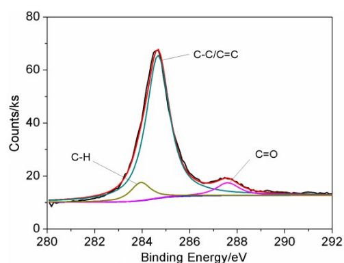
Fig. S2. XPS spectrum of the 1-FP/rGO: high resolution scans for C 1s.
