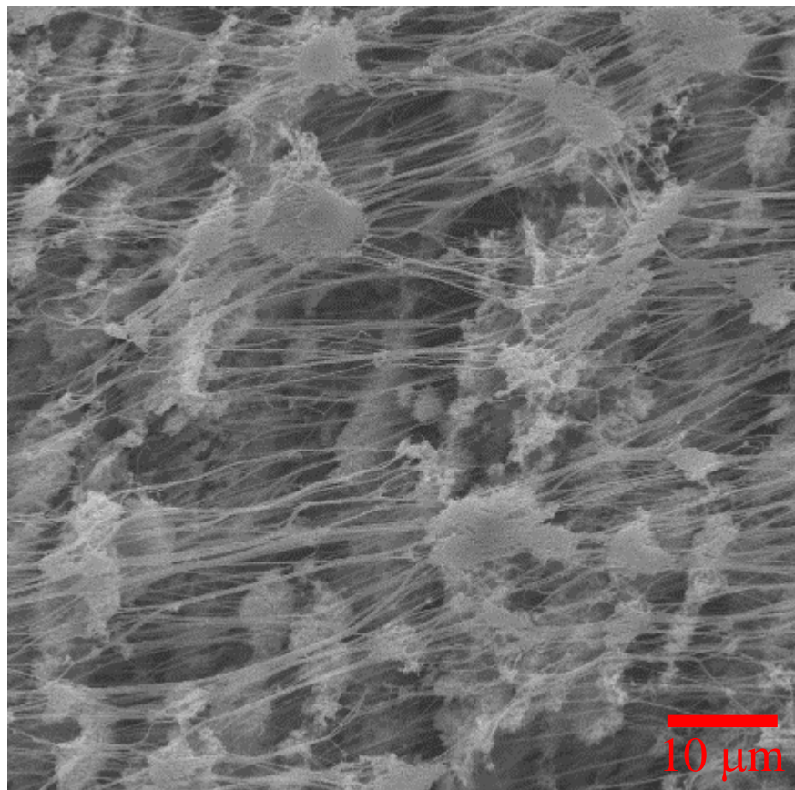
Fig. S1 The scanning electron microscopy image of stretched PTFE tape illustrates the porous structure.
