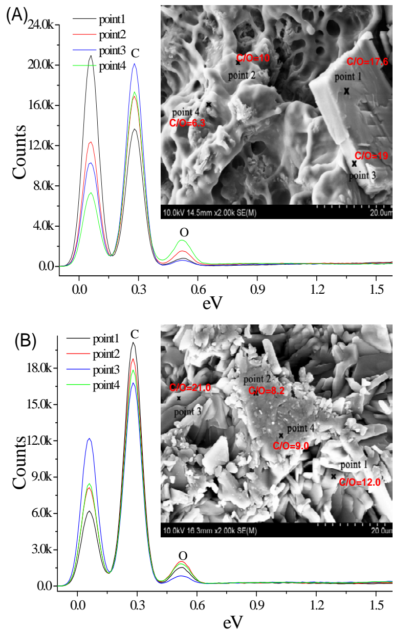
Figure S2. SEM/EDS elemental spectrum of (A) PySMPU-0.2OOBA and (B) PySMPU-1.0OOBA
