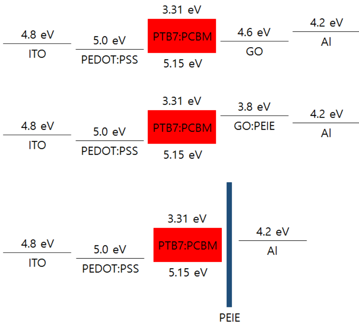
Figure S1. Energy levels of GO, GO:PEIE, and PEIE based conventional organic solar cells.
