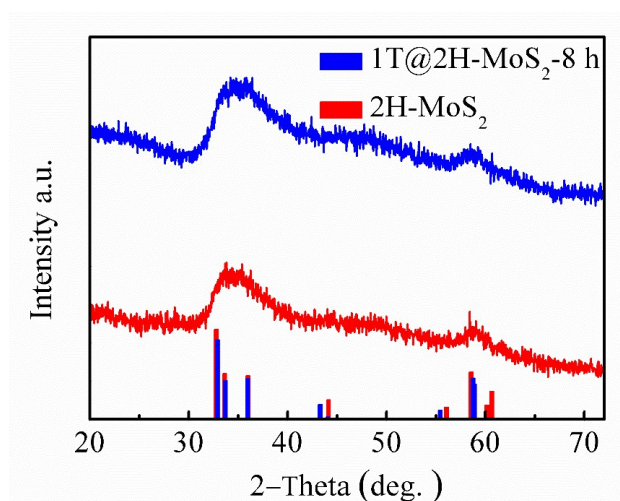
Figure S1: XRD patterns for sample 2H-MoS 2 and 1T@2H-MoS 2 nanosheets.
