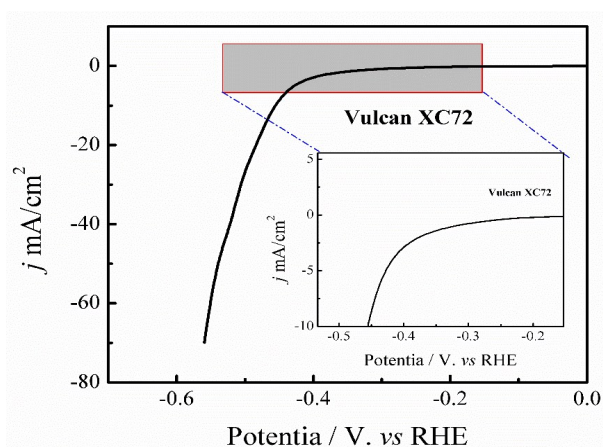
Figure S2: Polarization curve for Vulcan XC72 used in our case.
