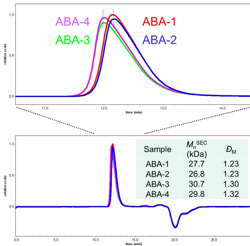
Figure S3. Overlaid SEC traces of triblock copolymers with their uncorrected polystyrene equivalent molar mass ( M_n^{SEC} ) and molar-mass dispersity ( D_M ) values listed.
