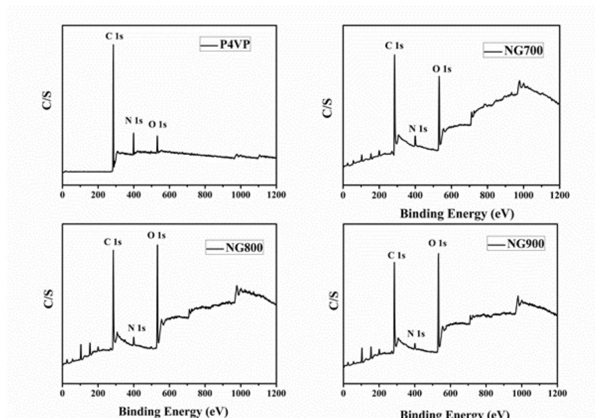
Figure S1. XPS spectra of P4VP, NG700, NG800 and NG900, respectively.
