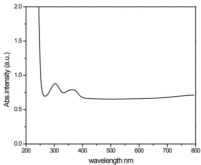
Figure 1 absorption spectra for ZnO NRAs
