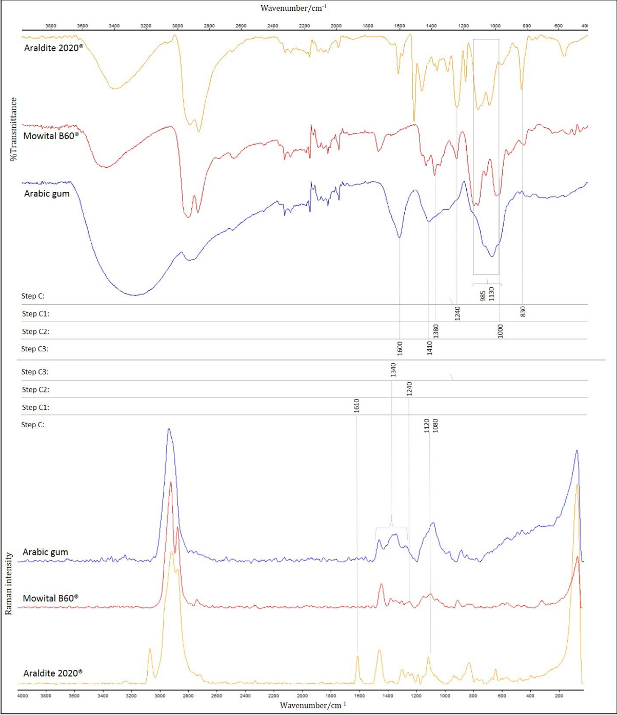
S4: Infrared and Raman spectra (1064nm) of Araldite 2020 ® , Mowital B60 ® and arabic gum
