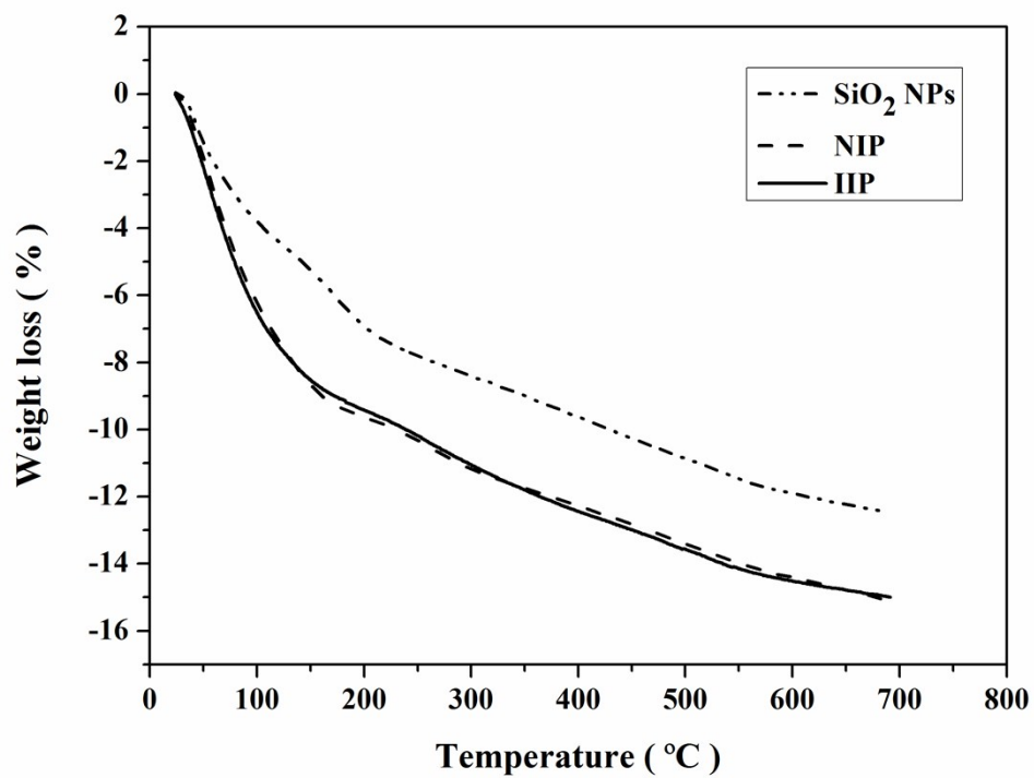
Fig.S1 Thermogravimetric analysis of SiO 2 NPs, SiO 2 @Se(IV)-IIPS and NIPs.
