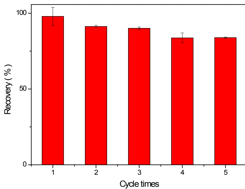
Fig.S5 Adsorption-desorption cycle of SiO 2 @Se (IV)-IIPs.
