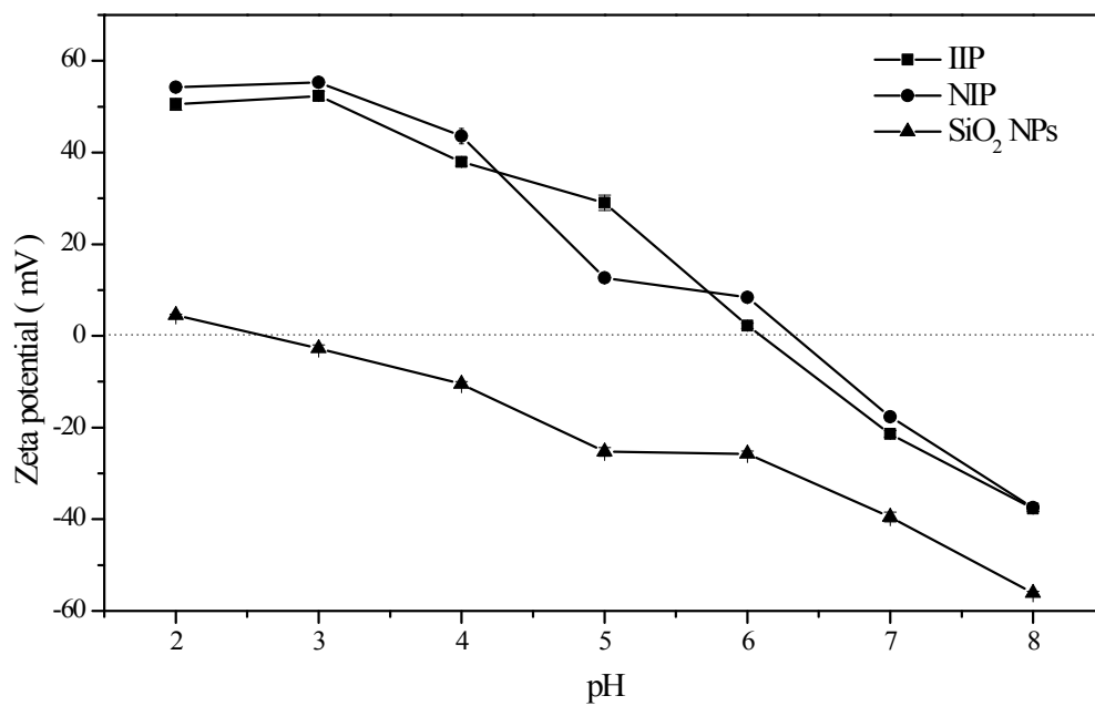
Fig.S2 Zeta potentials of SiO 2 NP, SiO 2 @Se(IV)-IIPs and NIPs.
