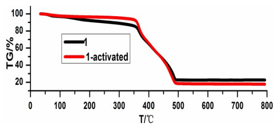
Fig. S1 The TG plots of 1 and activated samples.
