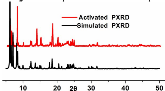
Fig. S2 The PXRD patterns simulated from crystal data of 1 , and of activated samples.
