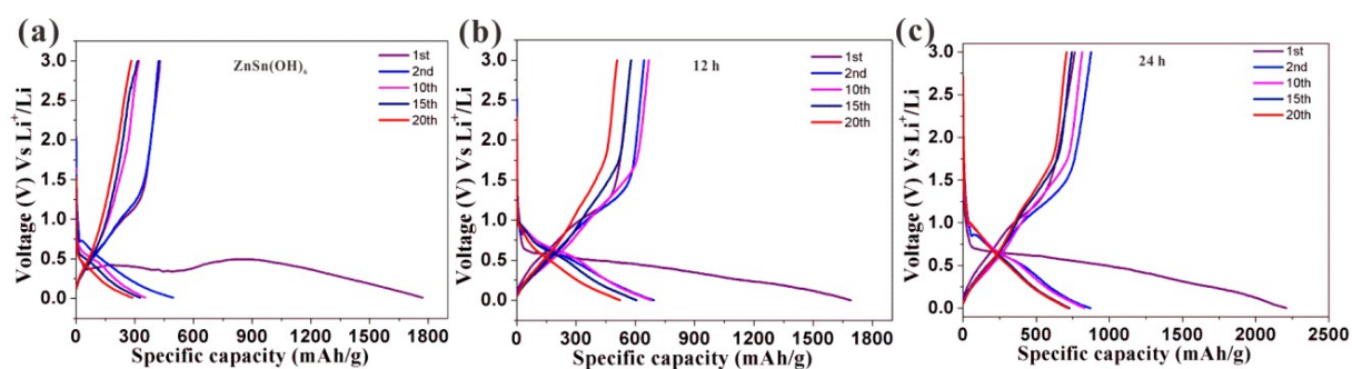
Fig. S1 Galvanostatic discharge-charge curves of three different samples at a rate of 100 \text{ mA g}^{-1} : (a) \text{ZnSn}(\text{OH})_6 ; (b) secondary-growth for 12 h; (c) secondary-growth for 24 h.
