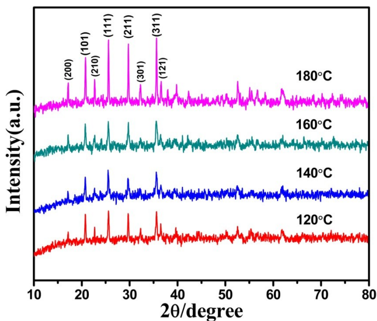
Figure S1. XRD patterns of the LFP/C-5 samples prepared under different reaction temperature.
