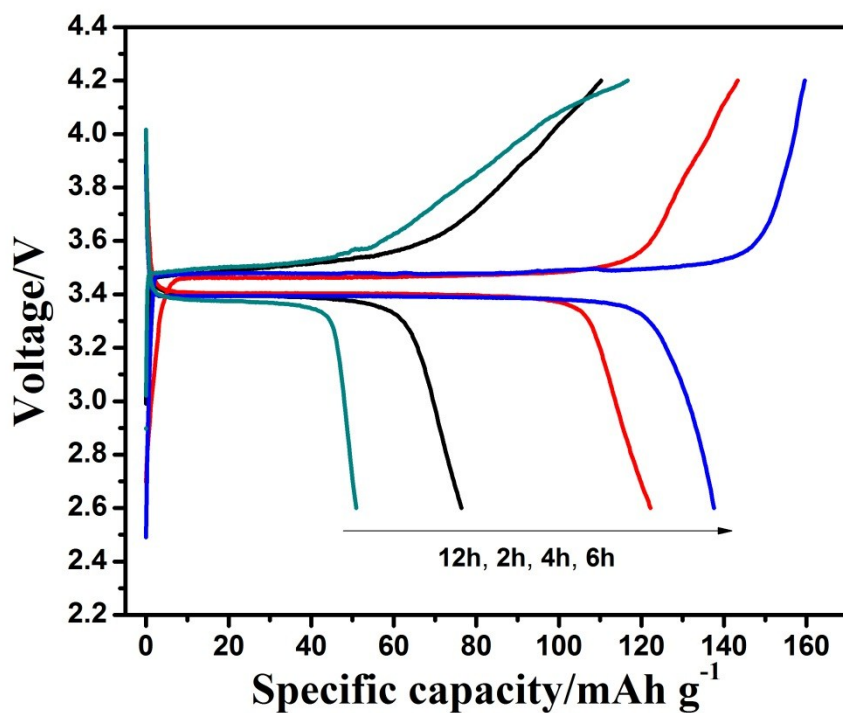
Figure S6. First charge/discharge curves of prepared by different reaction time.
