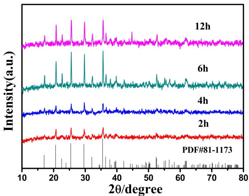
Figure S2. XRD patterns of the LFP/C-5 samples prepared with different reaction time.
