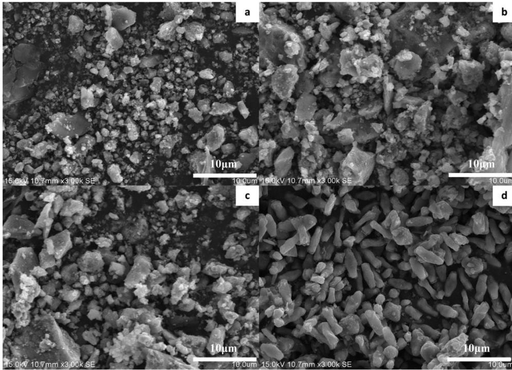
Figure S3. SEM images of LFP/C-5 samples prepared by various reaction temperature: (a) 120°C, (b) 140°C, (c) 160°C and (d) 180°C, respectively.
