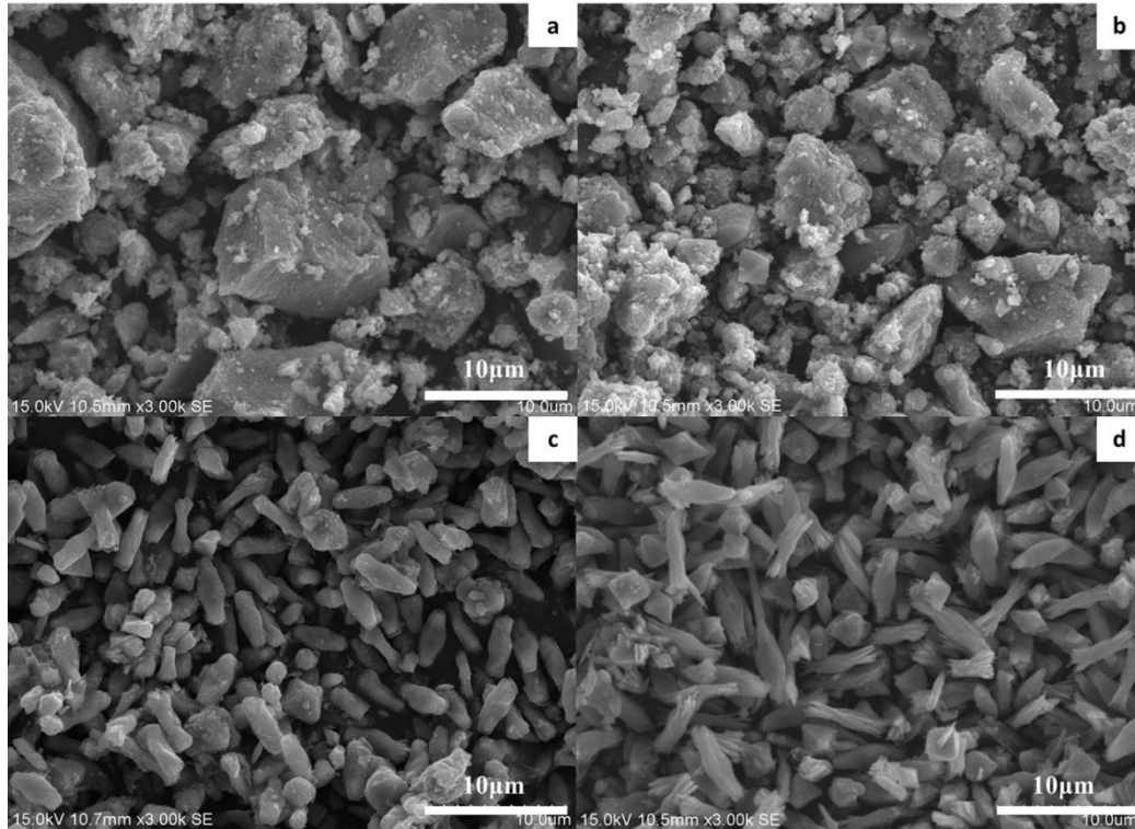
Figure S4. SEM images of LFP/C-5 samples prepared by various reaction time: (a) 2h, (b) 4h, (c) 6h and (d) 12h, respectively.
