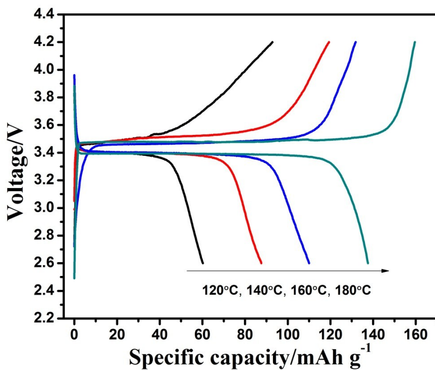
Figure S5. First charge/discharge curves of prepared by different reaction temperature.
