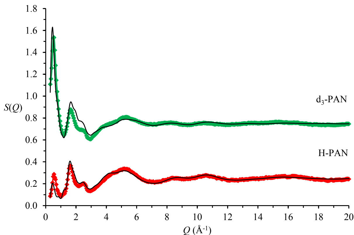
Figure S1. Measured (coloured diamonds) and EPSR fits (black lines) for pure propylammonium nitrate, PAN
