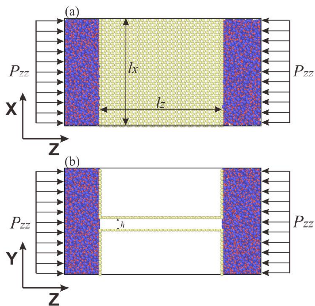
Figure S1. Configuration of simulation model: xz plane (a) and yz plane (b), similar to that shown in the Ref. 12. The red, blue, and yellow balls denote the hydrogen, oxygen, and carbon atoms, respectively. The black rectangle frame is the simulation box.
