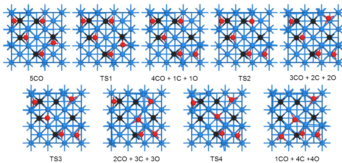
Figure S5: Structures of 5CO dissociation on Mo(100) surface.
