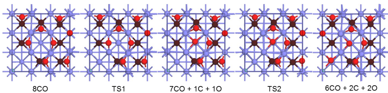
Fig. S8: Structures of 8CO dissociation on Mo(100) surface.
