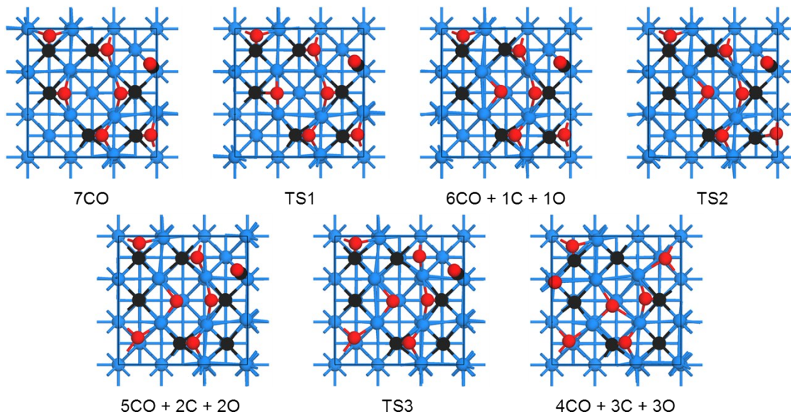
Figure S7: Structures of 7CO dissociation on Mo(100) surface.
