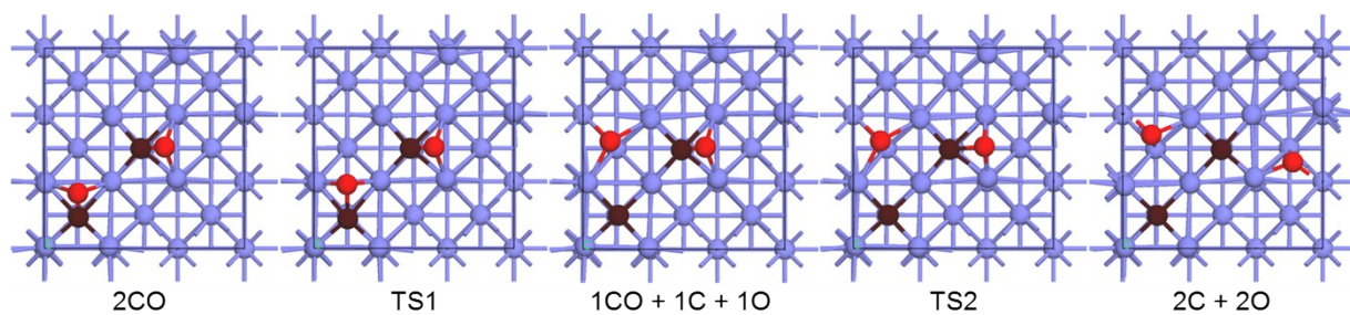
Fig. S2: Structures of 2CO dissociation on Mo(100) surface.
