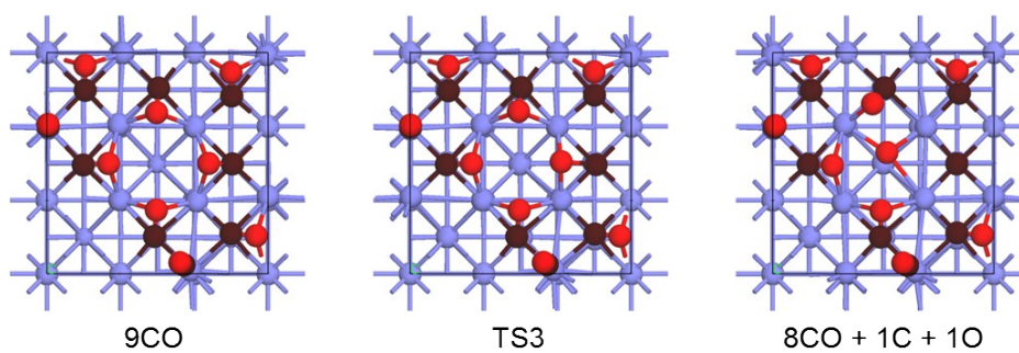
Fig. S9: Structures of 9CO dissociation on Mo(100) surface.
