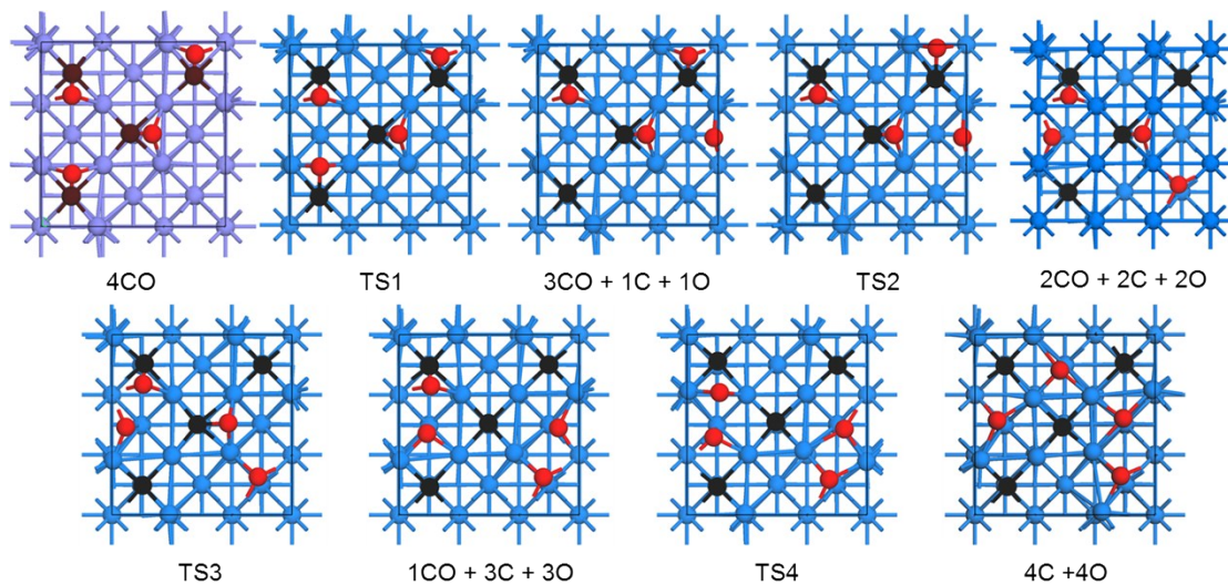
Figure S4: Structures of 4CO dissociation on Mo(100) surface.
