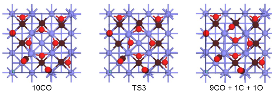
Fig. S10: Structures of 10CO dissociation on Mo(100) surface.
