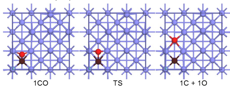
Fig. S1: Structures of 1CO dissociation on Mo(100) surface.
