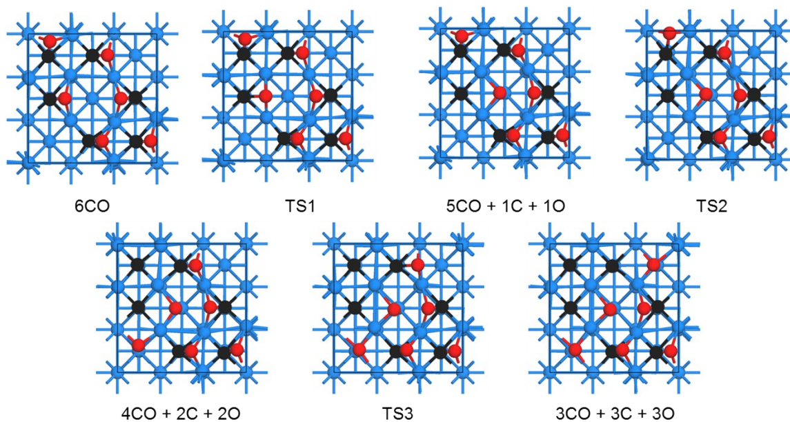
Figure S6: Structures of 6CO dissociation on Mo(100) surface.
