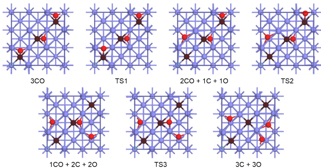
Fig. S3: Structures of 3CO dissociation on Mo(100) surface.
