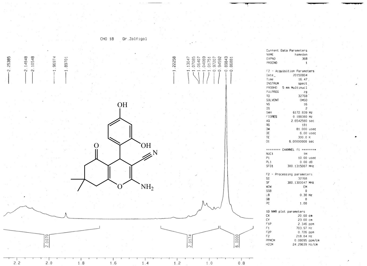
Fig S37. The ^1\text{H} NMR spectrum of 2-amino-4-(2,4-dihydroxyphenyl)-7,7-dimethyl-5-oxo-5,6,7,8-tetrahydro-4H-chromene-3-carbonitrile (Table 3, entry 18)
