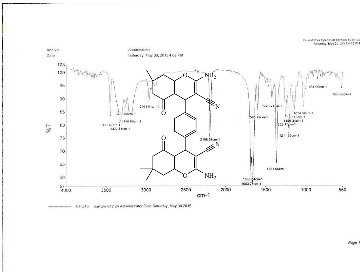
Fig S25. The IR spectrum of 4,4'-(1,4-phenylene)bis(2-amino-7,7-dimethyl-5-oxo-5,6,7,8-tetrahydro-4H-chromene-3-carbonitrile) (Table 3, entry 13)
