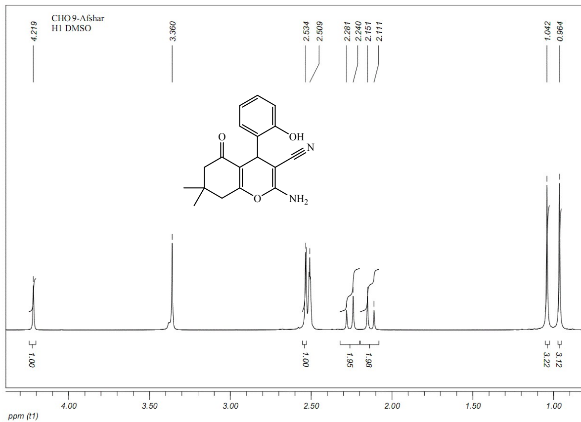
Fig S8. The ^1\text{H} NMR spectrum of 2-amino-4-(2-hydroxyphenyl)-7,7-dimethyl-5-oxo-5,6,7,8-tetrahydro-4H-chromene-3-carbonitrile (Table 3, entry 9)
