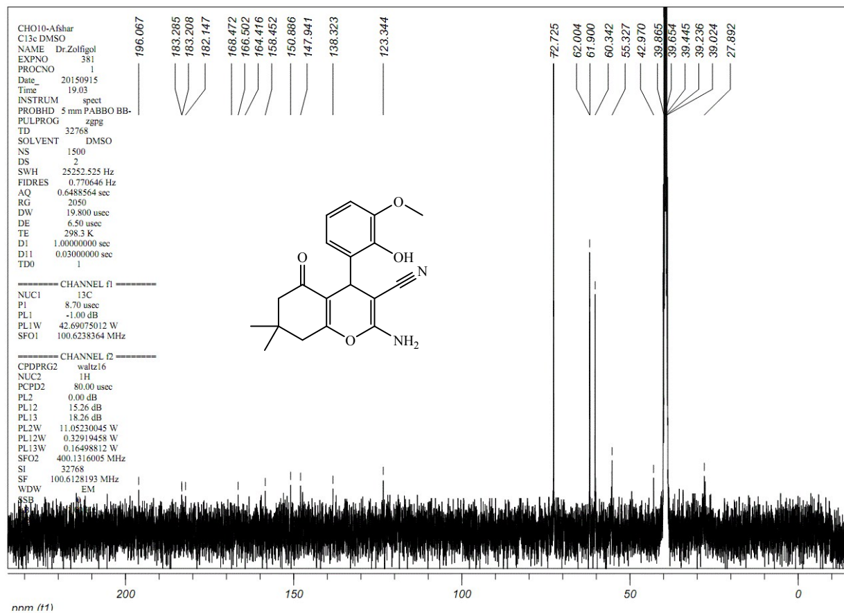
Fig S15. The ^{13}\text{C} NMR spectrum of 2-amino-4-(2-hydroxy-3-methoxyphenyl)-7,7-dimethyl-5-oxo-5,6,7,8-tetrahydro-4H-chromene-3-carbonitrile (Table 3, entry 10)
