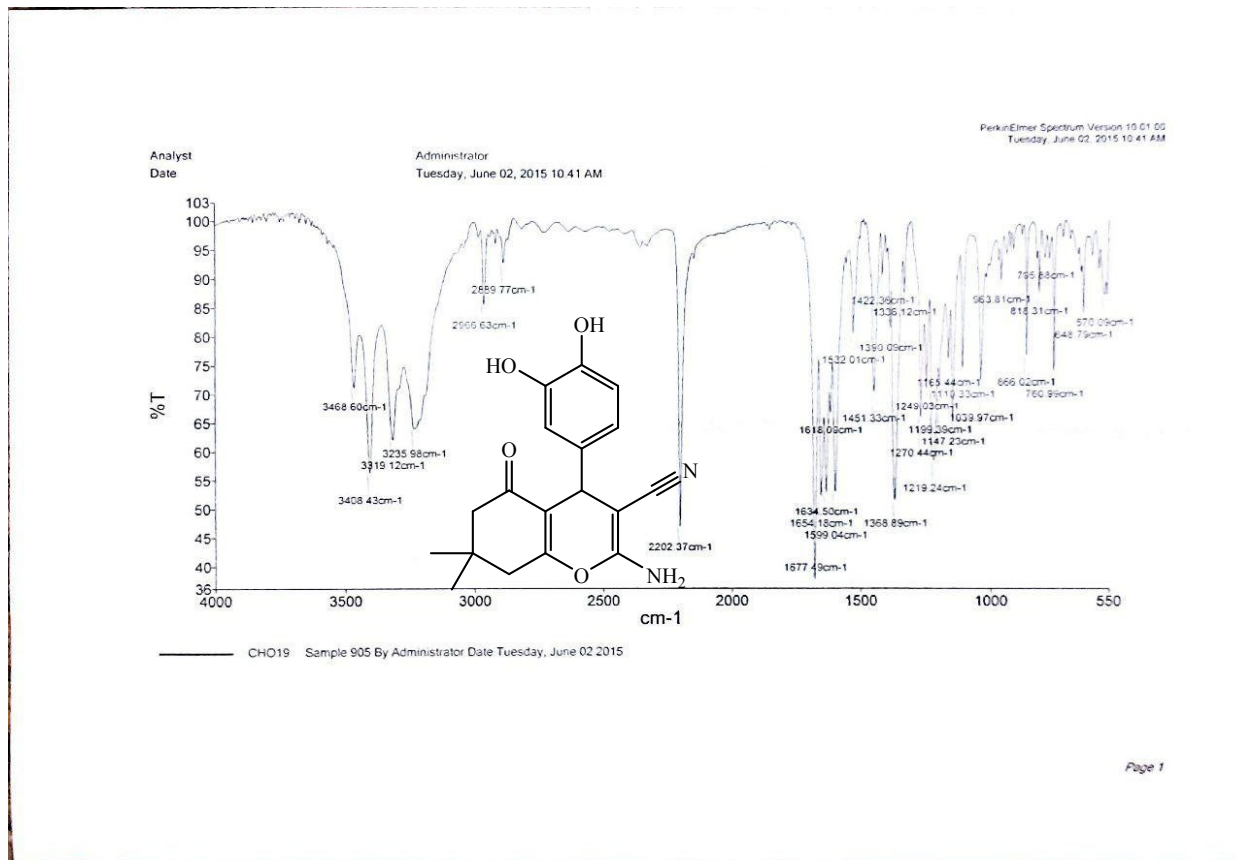
Fig S40. The IR spectrum of 2-amino-4-(3,4-dihydroxyphenyl)-7,7-dimethyl-5-oxo-5,6,7,8-tetrahydro-4H-chromene-3-carbonitrile (Table 3, entry 19)
