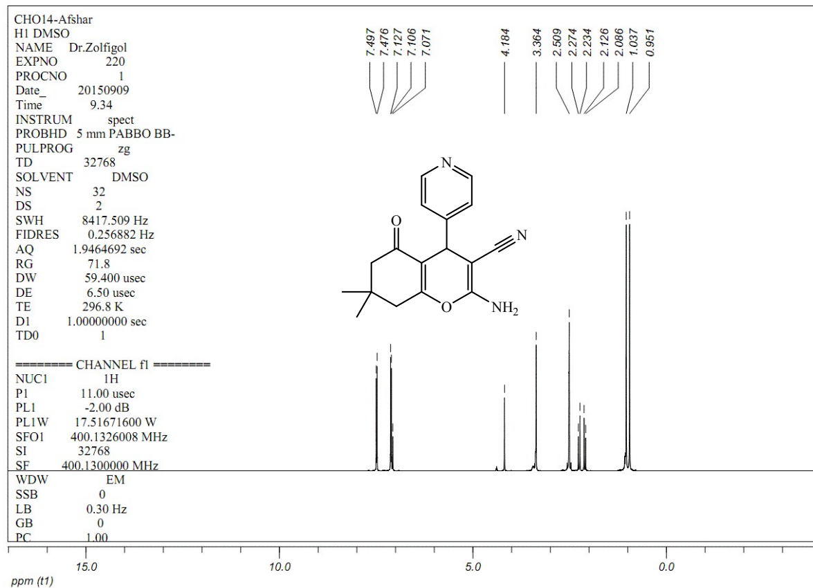
Fig S31. The ^1\text{H} NMR spectrum of 2-amino-7,7-dimethyl-5-oxo-4-(pyridin-4-yl)-5,6,7,8-tetrahydro-4H-chromene-3-carbonitrile (Table 3, entry 14)
