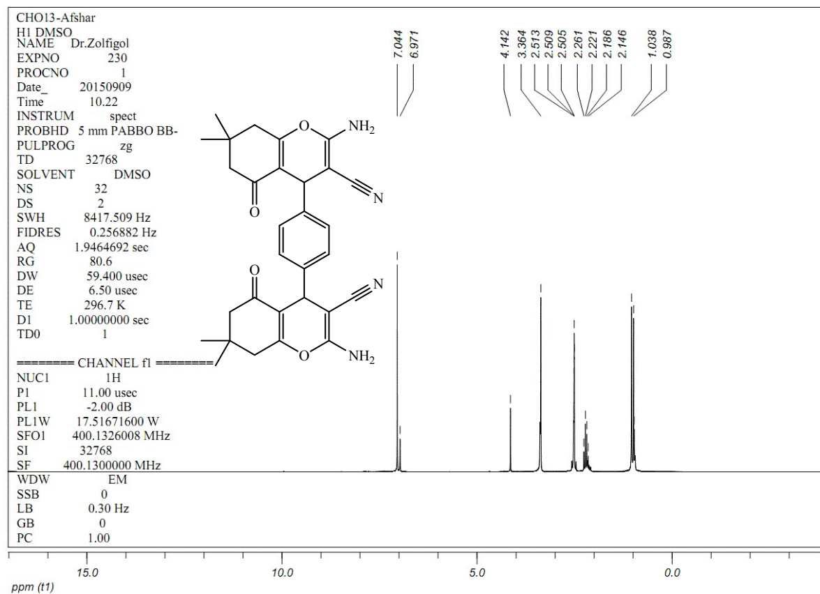
Fig S26. The ^1\text{H} NMR spectrum of 4,4'-(1,4-phenylene)bis(2-amino-7,7-dimethyl-5-oxo-5,6,7,8-tetrahydro-4H-chromene-3-carbonitrile) (Table 3, entry 13)
