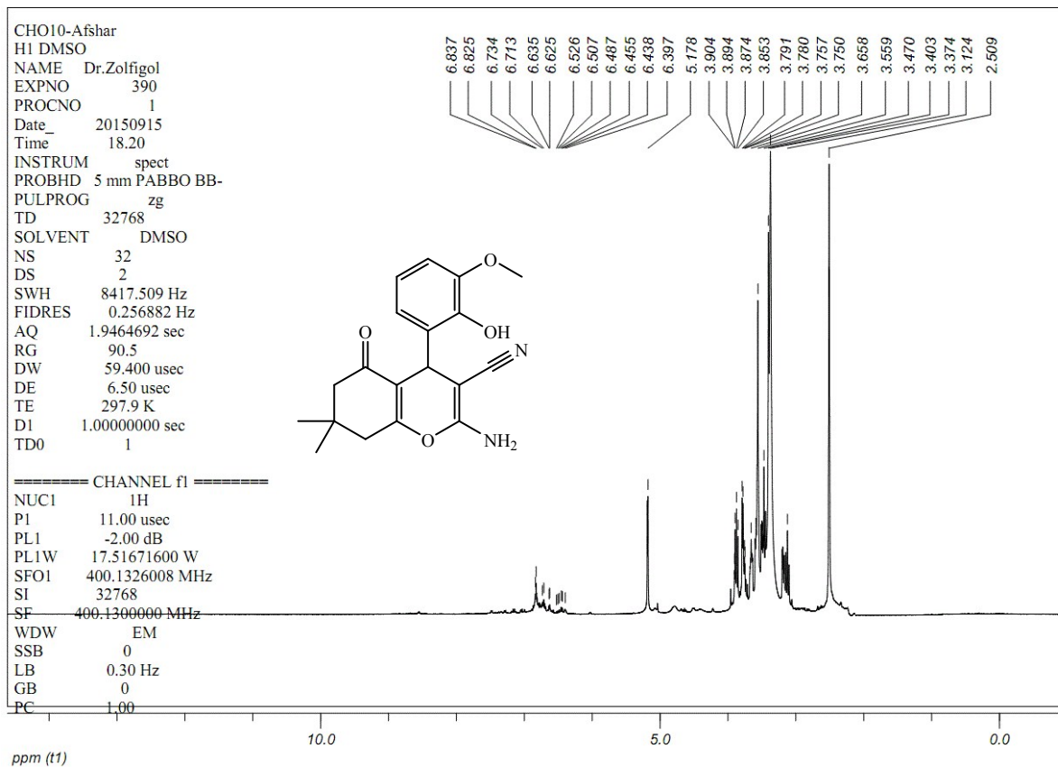
Fig S12. The ^1\text{H} NMR spectrum of 2-amino-4-(2-hydroxy-3-methoxyphenyl)-7,7-dimethyl-5-oxo-5,6,7,8-tetrahydro-4H-chromene-3-carbonitrile (Table 3, entry 10)
