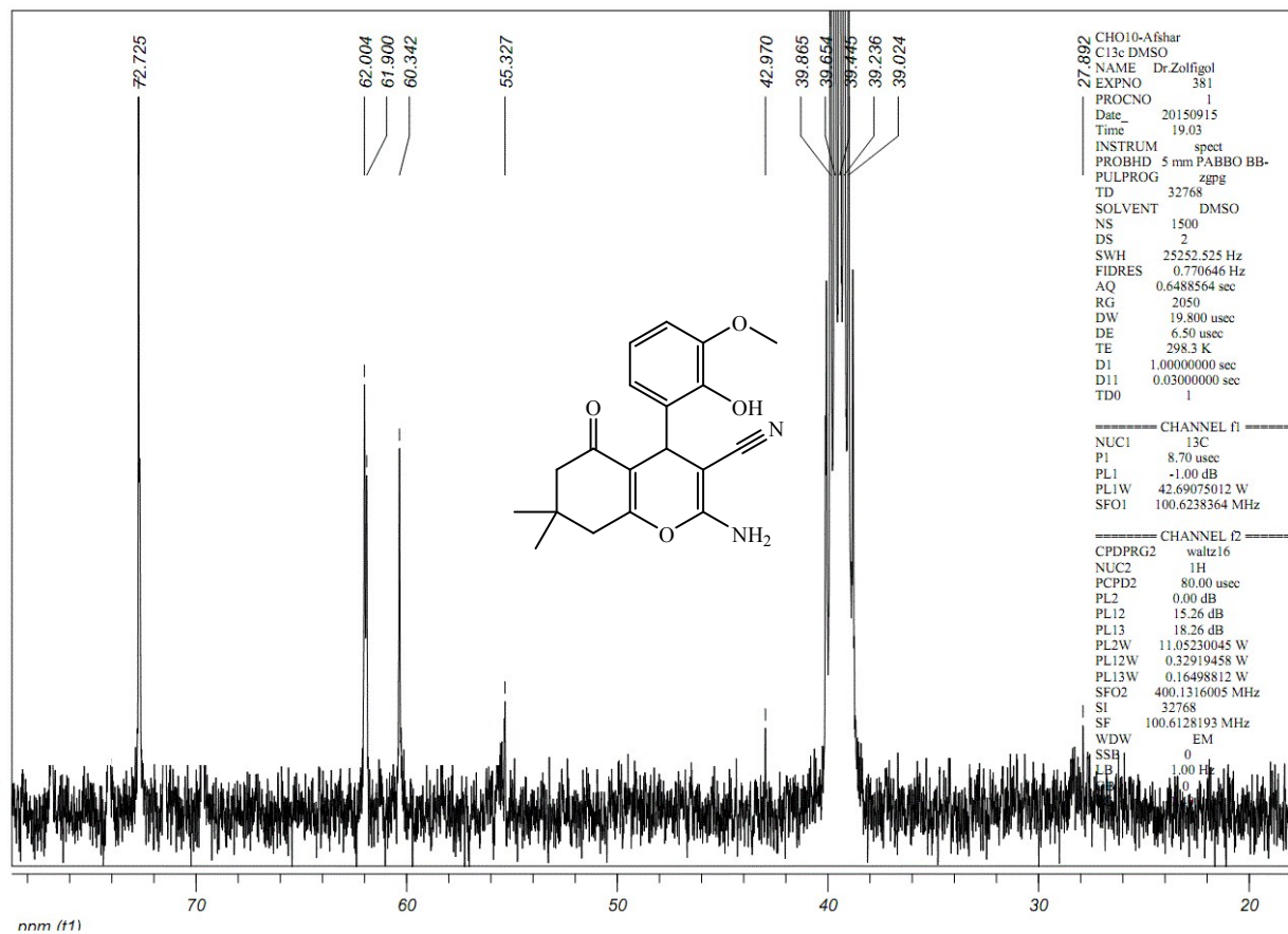
Fig S16. The ^{13}\text{C} NMR spectrum of 2-amino-4-(2-hydroxy-3-methoxyphenyl)-7,7-dimethyl-5-oxo-5,6,7,8-tetrahydro-4H-chromene-3-carbonitrile (Table 3, entry 10)
