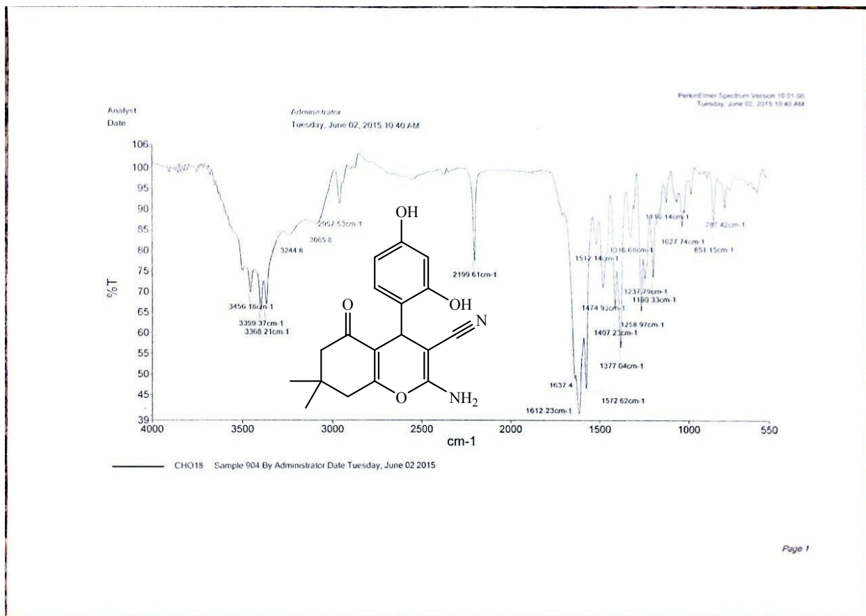
Fig S35. The IR spectrum of 2-amino-4-(2,4-dihydroxyphenyl)-7,7-dimethyl-5-oxo-5,6,7,8-tetrahydro-4H-chromene-3-carbonitrile (Table 3, entry 18)
