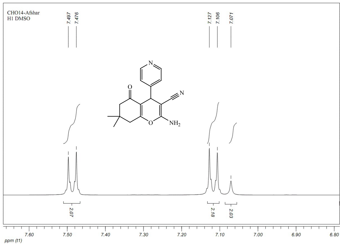
Fig S33. The ^1\text{H} NMR spectrum of 2-amino-7,7-dimethyl-5-oxo-4-(pyridin-4-yl)-5,6,7,8-tetrahydro-4H-chromene-3-carbonitrile (Table 3, entry 14)
