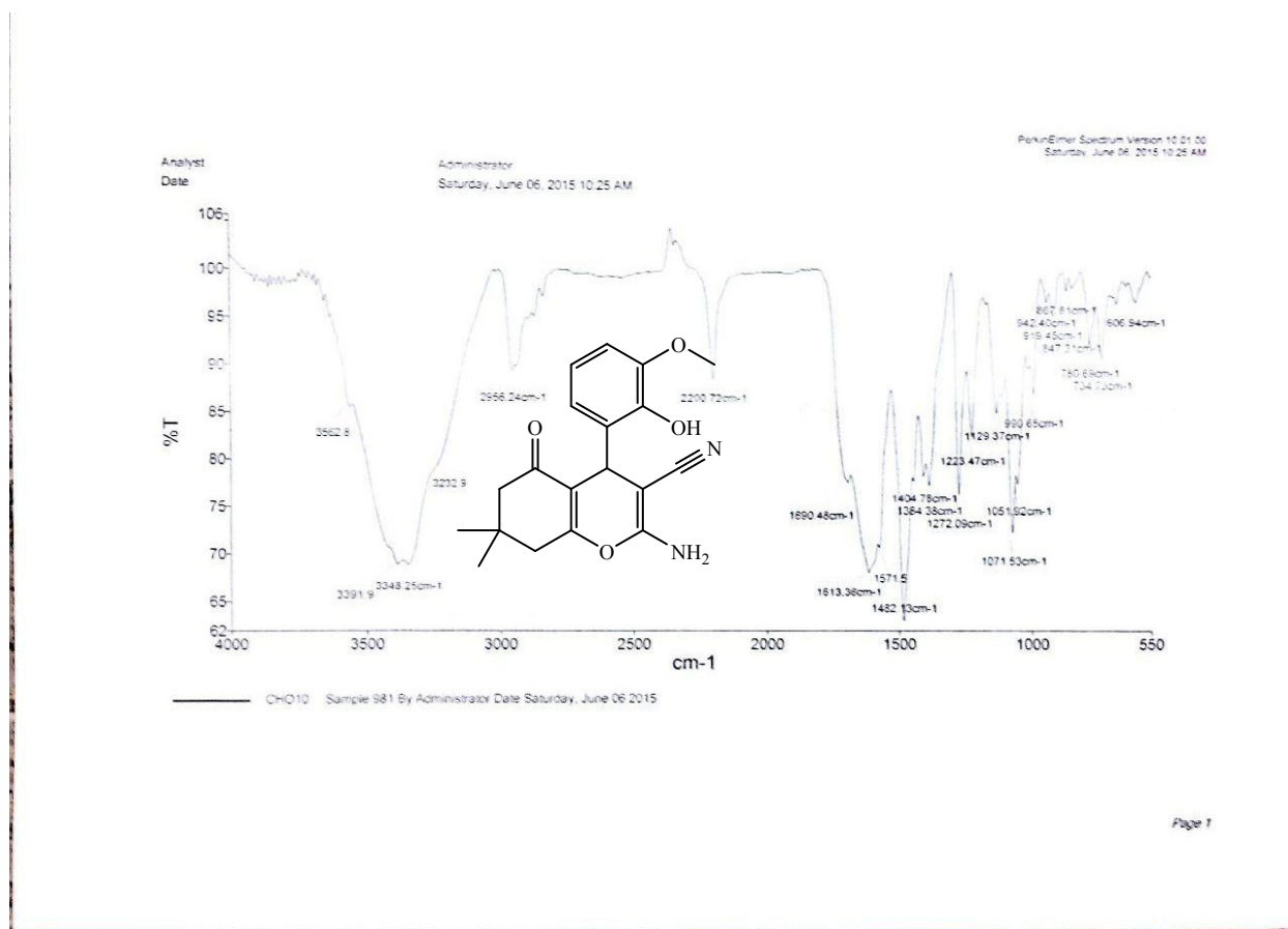
Fig S11. The IR spectrum of 2-amino-4-(2-hydroxy-3-methoxyphenyl)-7,7-dimethyl-5-oxo-5,6,7,8-tetrahydro-4H-chromene-3-carbonitrile (Table 3, entry 10)
