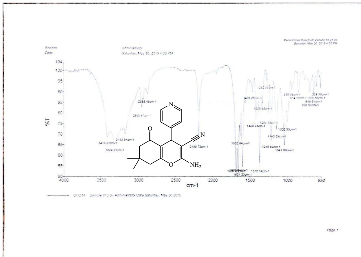
Fig S30. The IR spectrum of 2-amino-7,7-dimethyl-5-oxo-4-(pyridin-4-yl)-5,6,7,8-tetrahydro-4H-chromene-3-carbonitrile (Table 3, entry 14)
