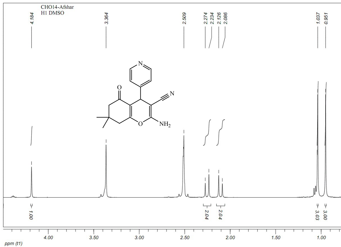
Fig S32. The ^1\text{H} NMR spectrum of 2-amino-7,7-dimethyl-5-oxo-4-(pyridin-4-yl)-5,6,7,8-tetrahydro-4H-chromene-3-carbonitrile (Table 3, entry 14)
