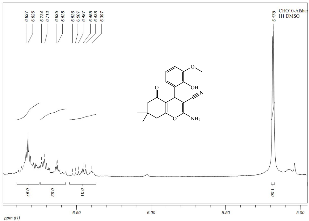
Fig S14. The ^1\text{H} NMR spectrum of 2-amino-4-(2-hydroxy-3-methoxyphenyl)-7,7-dimethyl-5-oxo-5,6,7,8-tetrahydro-4H-chromene-3-carbonitrile (Table 3, entry 10)
