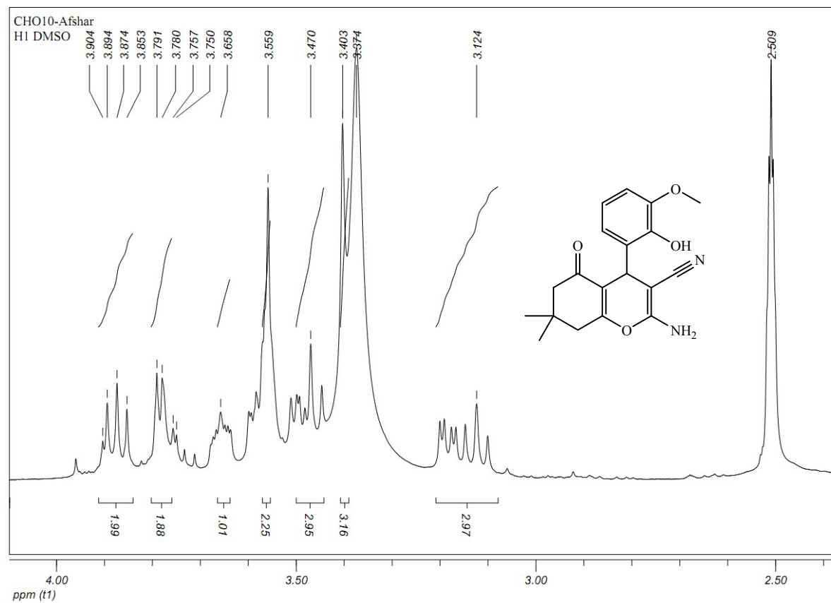
Fig S13. The ^1\text{H} NMR spectrum of 2-amino-4-(2-hydroxy-3-methoxyphenyl)-7,7-dimethyl-5-oxo-5,6,7,8-tetrahydro-4H-chromene-3-carbonitrile (Table 3, entry 10)
