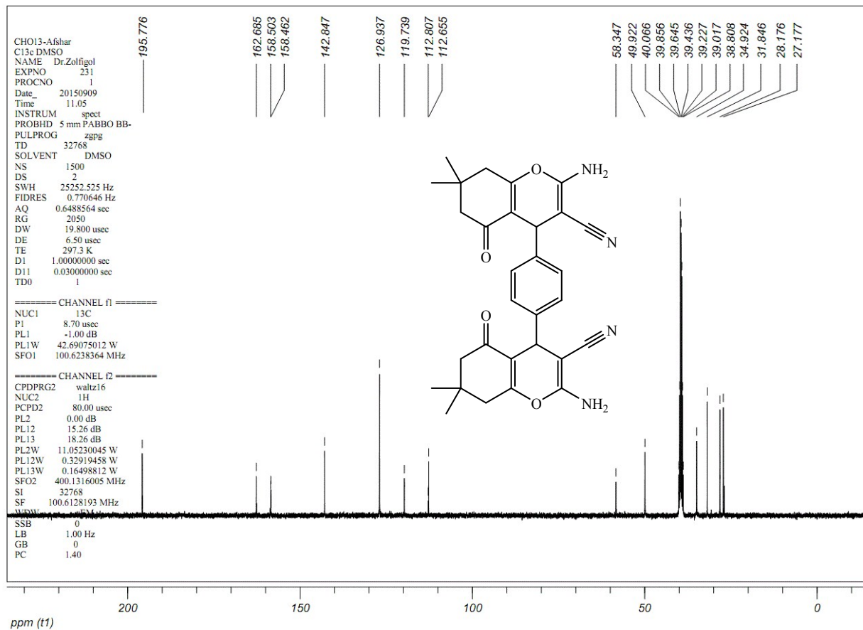
Fig S29. The ^{13}\text{C} NMR spectrum of 4,4'-(1,4-phenylene)bis(2-amino-7,7-dimethyl-5-oxo-5,6,7,8-tetrahydro-4H-chromene-3-carbonitrile) (Table 3, entry 13)
