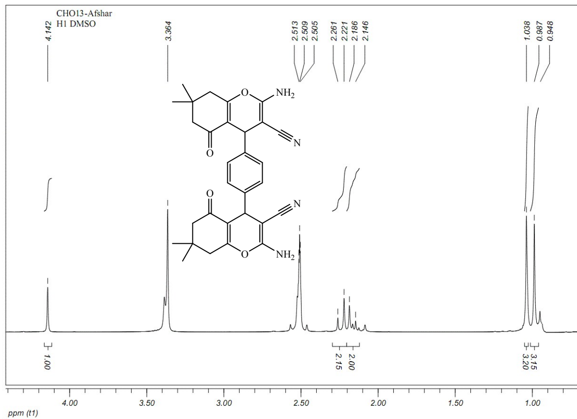
Fig S27. The ^1\text{H} NMR spectrum of 4,4'-(1,4-phenylene)bis(2-amino-7,7-dimethyl-5-oxo-5,6,7,8-tetrahydro-4H-chromene-3-carbonitrile) (Table 3, entry 13)
