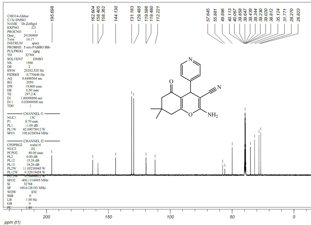
Fig S34. The ^{13}\text{C} NMR spectrum of 2-amino-7,7-dimethyl-5-oxo-4-(pyridin-4-yl)-5,6,7,8-tetrahydro-4H-chromene-3-carbonitrile (Table 3, entry 14)
