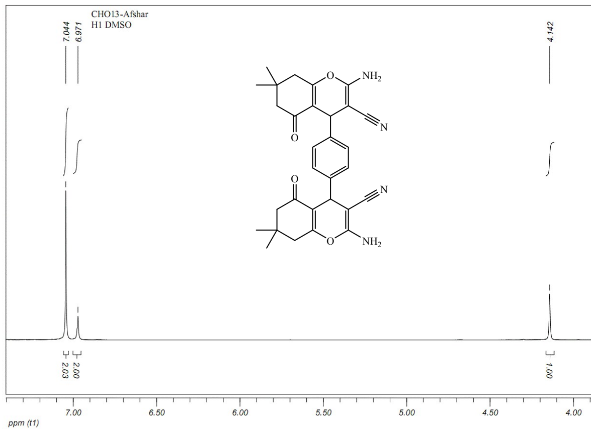
Fig S28. The ^1\text{H} NMR spectrum of 4,4'-(1,4-phenylene)bis(2-amino-7,7-dimethyl-5-oxo-5,6,7,8-tetrahydro-4H-chromene-3-carbonitrile) (Table 3, entry 13)
