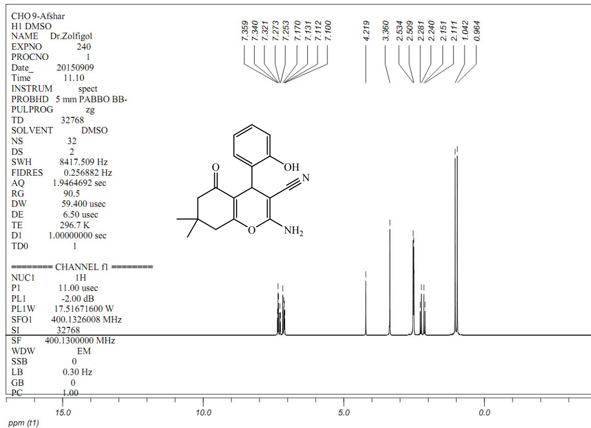
Fig S7. The ^1\text{H} NMR spectrum of 2-amino-4-(2-hydroxyphenyl)-7,7-dimethyl-5-oxo-5,6,7,8-tetrahydro-4H-chromene-3-carbonitrile (Table 3, entry 9)
