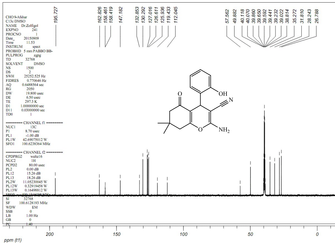
Fig S10. The ^{13}\text{C} NMR spectrum of 2-amino-4-(2-hydroxyphenyl)-7,7-dimethyl-5-oxo-5,6,7,8-tetrahydro-4H-chromene-3-carbonitrile (Table 3, entry 9)
