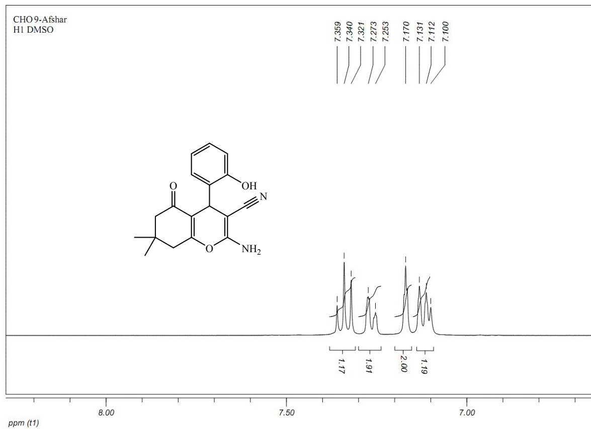
Fig S9. The ^1\text{H} NMR spectrum of 2-amino-4-(2-hydroxyphenyl)-7,7-dimethyl-5-oxo-5,6,7,8-tetrahydro-4H-chromene-3-carbonitrile (Table 3, entry 9)
