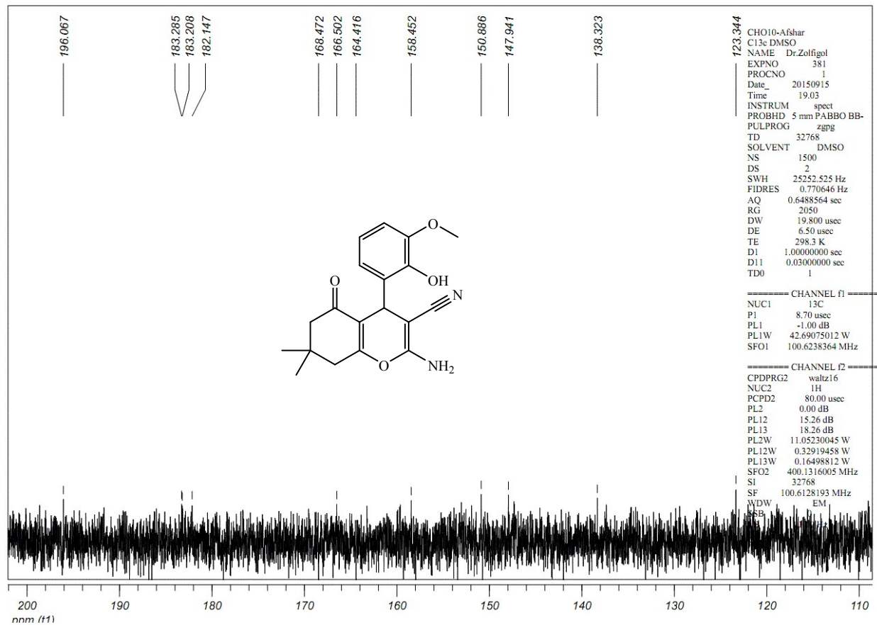
Fig S17. The ^{13}\text{C} NMR spectrum of 2-amino-4-(2-hydroxy-3-methoxyphenyl)-7,7-dimethyl-5-oxo-5,6,7,8-tetrahydro-4H-chromene-3-carbonitrile (Table 3, entry 10)
