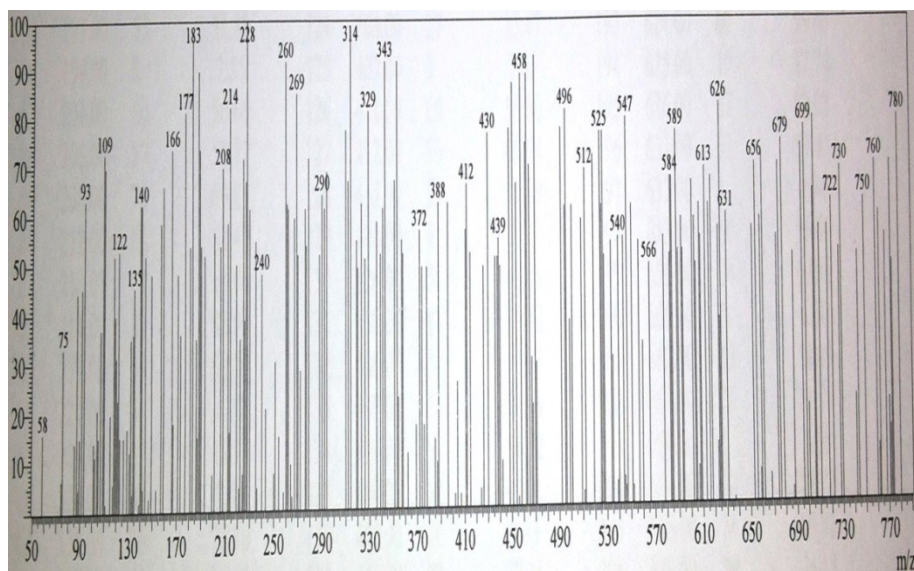
S2: The experimental, calculated IR spectrum and Mass spectrum of [(\text{PdL}_2)_2\mu\text{PPi}]\cdot\text{H}_2\text{O} complex (2).
