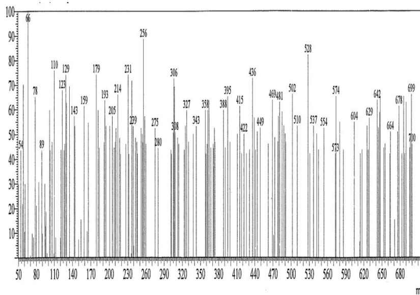
S3: The experimental, calculated IR spectrum and Mass spectrum of [(PdL 3 ) 2 μPPi].4H 2 O complex (3).
