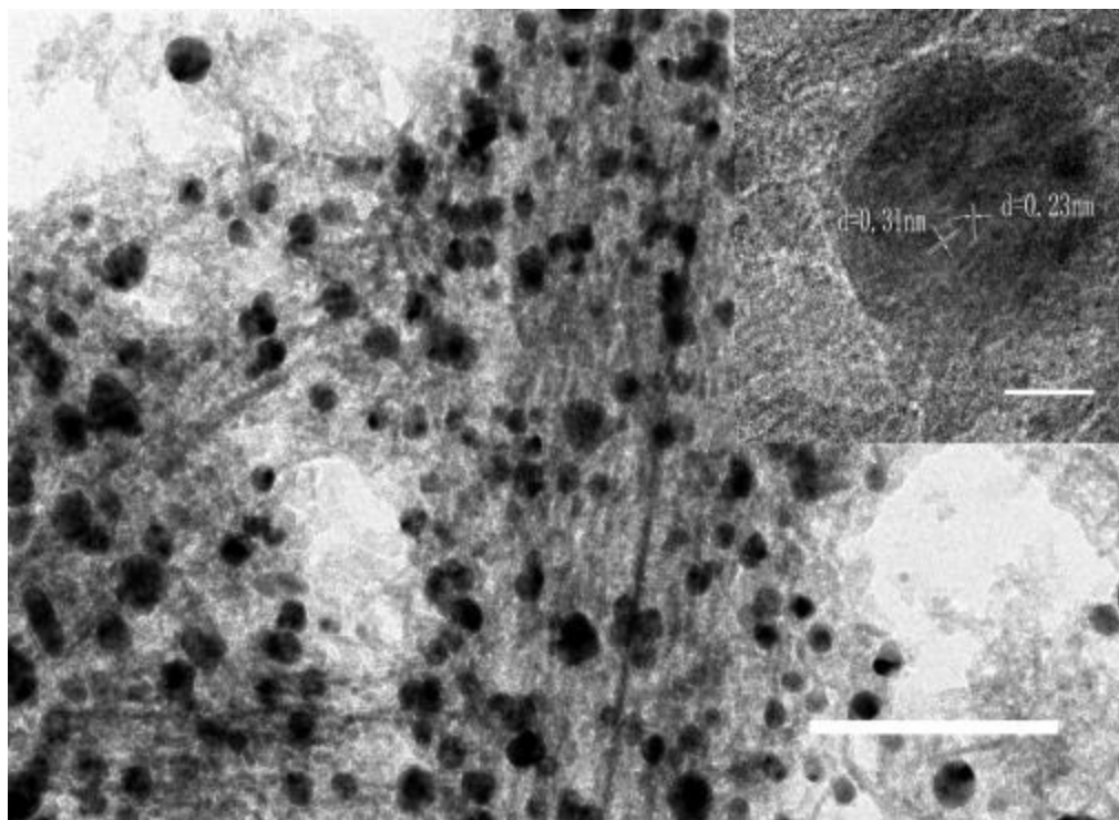
Figure S2 Transmission electron micrograph of Ag@PSMs-75; the inset is a HRTEM image of single Ag NPs anchored on the PSMs of sample Ag@PSMs-75.
