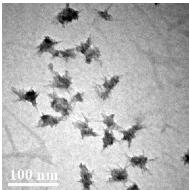
Figure S1. TEM image of CdSe NCs prepared from a control experiment using only Cd-BPA-Br precursors in the absence of Cd-BPA-P3HT.
