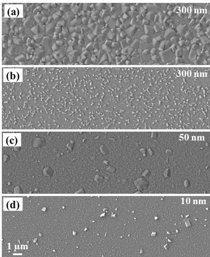
Figure S2 (a) SEM imaging results for sputter deposited Mo films sulfurized at 850°C for 30 min. In (a) the 300 nm Mo film sulfurized using 150 mg of S powder, and in (b), (c) and (d) the 300, 50 and 10 nm films, respectively, sulfurized using 300 mg of S powder. (High magnification images for samples presented in panel (b) and (c) are provided in Figure 1 which confirm the nanosheet presence.)
