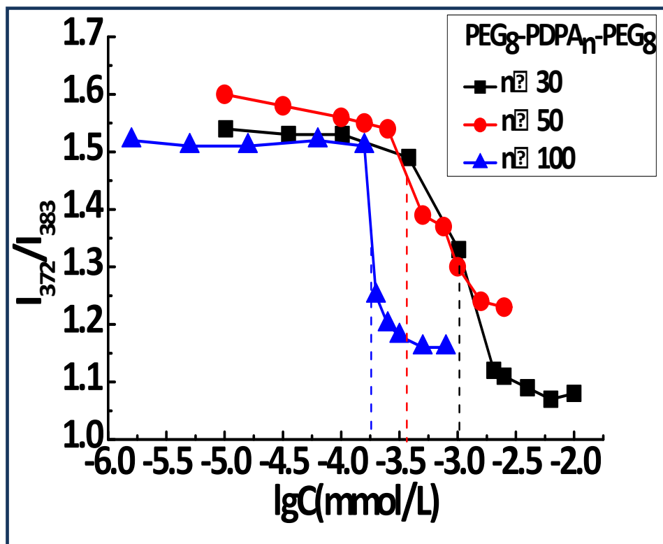
S1: The fluorescence intensity ratio ( I_{372}/I_{383} ) versus logarithm of critical micelles concentrations (PEG 8 -PDPA 30 -PEG 8 , PEG 8 -PDPA 50 -PEG 8 and PEG 8 -PDPA 100 -PEG 8 ).
